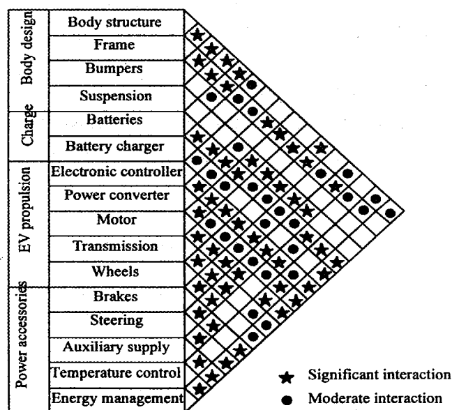
Figure 22: Subsystem interactions
