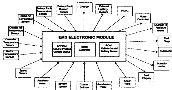
Figure 20: Energy management system
