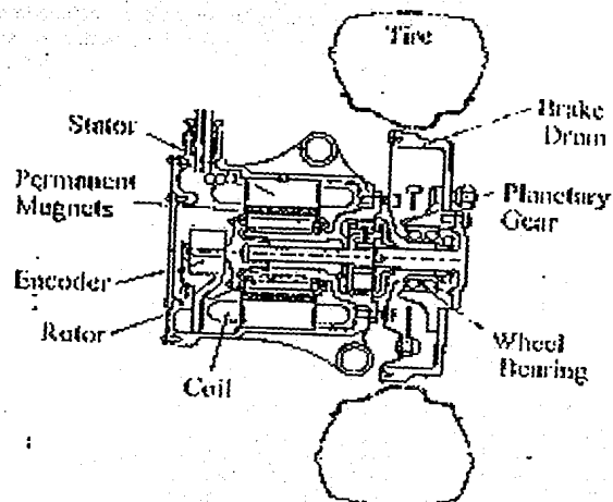
Figure 13: Wheel motor
