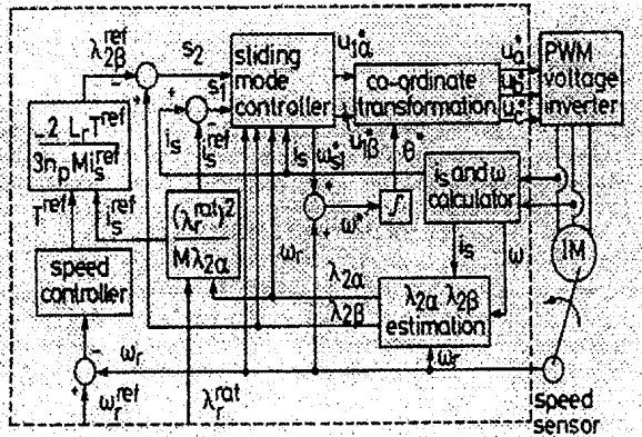
Figure 14: Novel sliding mode control of induction motor drive
