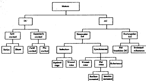
A classification of motors for electric propulsion is shown in Figure 8, where the shaded motor types have been accepted for EVs. Both the GM Impact/Impact 4 and Nissan FEV employ the induction motor, while both the BMW E1/E2 and U2001 use the PM brushless DC motor. The dual induction motors in the Nissan FEV possess a rated output of 20 kW and starting torque of 95.5 Nm, while the PM brushless DC motor in the BMW E1 has 32 kW and 150 Nm. On the other hand, the other motor types are also employed in EVs, such as the PM synchronous motor in the Ford/GE ETX-II, the switched reluctance motor in the Chloride Lucas, the DC series motor in the Daihatsu Hijet, the DC shunt motor in the Mazda Bongo, the DC separately excited motor in the Fiat 900E/E2, and the PM DC motor in the Suzuki Senior Tricycle.
