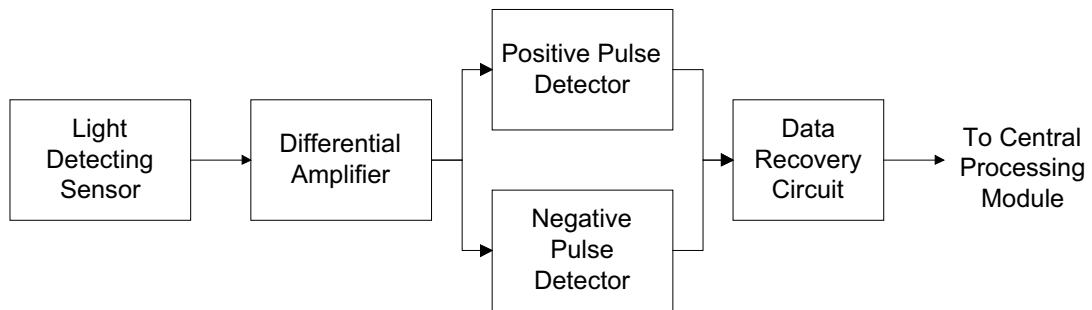
Figure 5. Visible light receiver
