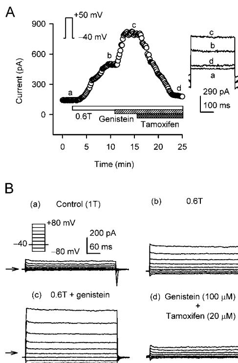
FIGURE 4. Tamoxifen blocks swelling- and genistein-induced current. (A) Time course of membrane current at +50 mV. I_{Cl.vol} activated upon switching from 1T to 0.6T and was augmented by 100 \mu M genistein. Tamoxifen (20 \mu M) substantially inhibited both the swelling- and genistein-induced currents. Currents at time points a–d at right. (B) Voltage-dependent currents in 1T control (a), 0.6T (b), 0.6T with 100 \mu M genistein (c), and 0.6T with genistein and 20 \mu M tamoxifen. Both the 0.6T- and genistein-stimulated currents were outwardly rectifying. Arrows indicate 0 current. Voltage protocols are shown in insets.
