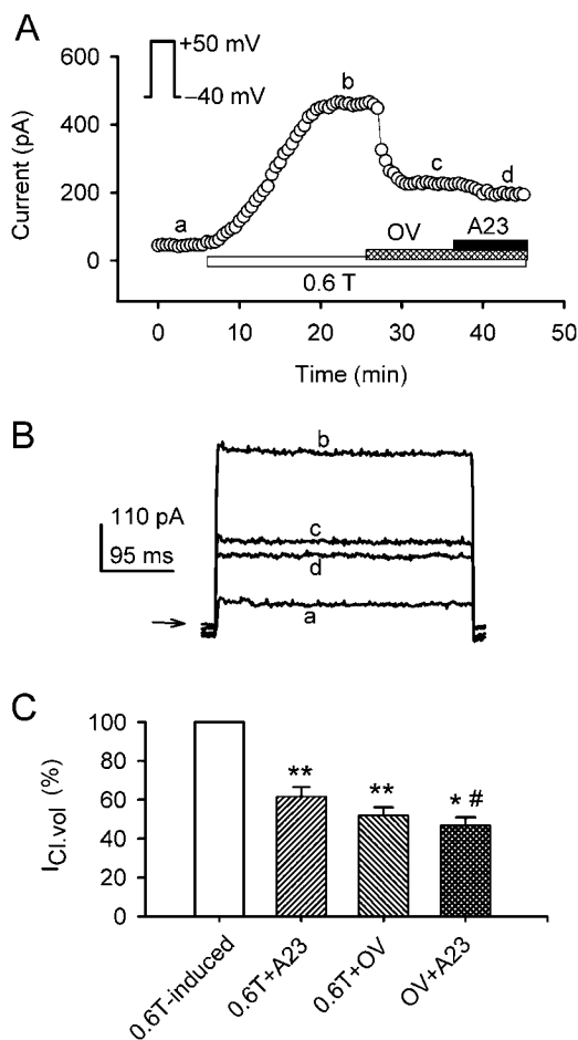
FIGURE 11. \text{VO}_4^{-3} (OV) antagonized the inhibition of I_{\text{Cl.vol}} by the typhostin A23. (A) Time course of current at +50 mV. I_{\text{Cl.vol}} was elicited by switching from 1T (a) to 0.6T (b) bath solution. Cells then were exposed to 1 mM \text{VO}_4^{-3} (OV, c) and \text{VO}_4^{-3} plus 100 \mu\text{M} A23 (d) in 0.6T. Pretreatment with \text{VO}_4^{-3} significantly diminished the block of I_{\text{Cl.vol}} by A23. Protocol is in inset. (B) Currents at time points a–d in A. (C) Histograms summarize effect of 100 \mu\text{M} A23, 1 mM \text{VO}_4^{-3} , and \text{VO}_4^{-3} plus 100 \mu\text{M} A23 on I_{\text{Cl.vol}} induced by swelling in 0.6T. ** P < 0.01 vs. 0.6T-induced I_{\text{Cl.vol}} ; * P < 0.05 vs. 0.6T with \text{VO}_4^{-3} ; # P < 0.01 vs. 0.6T with A23.
