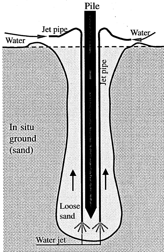
Fig. 1. Conventional jetting of water in the form of a cone from one nozzle at the toe of a jet pipe adjacent to a pile (modified from Tsinker 1988).
