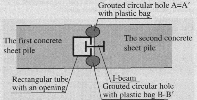
Fig. 10. Horizontal section showing the grouted two circular holes for sealing the open spaces in the rectangular tube and between two sheet piles.
