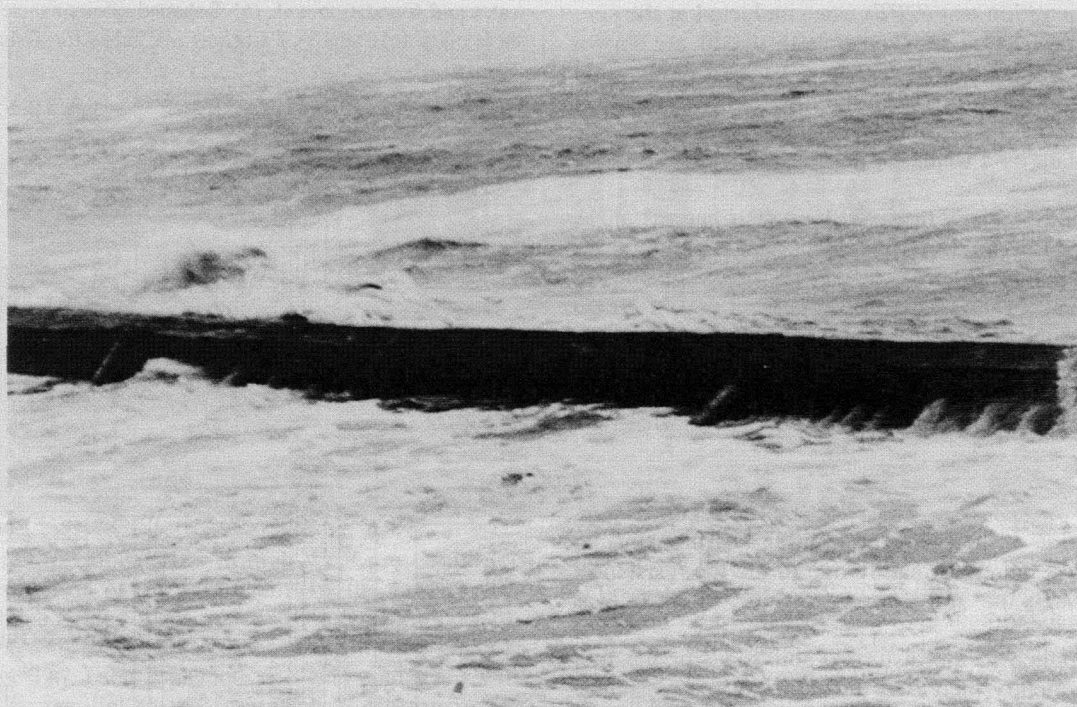
Fig. 21. Breakwater constructed with grouted jetted precast concrete sheet piling method in near shore of Bohai Sea, China.
