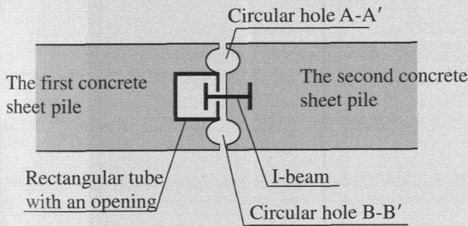
Fig. 9. Horizontal cross-section showing initial connection between two sheet piles before grouting.
