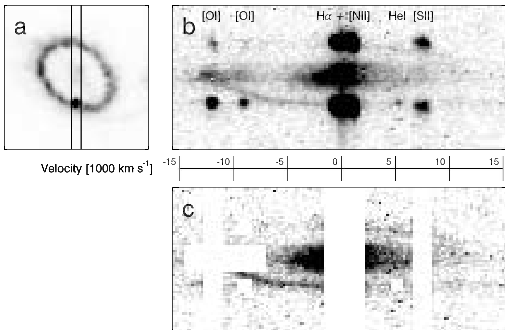
FIG. 3.—H \alpha line profile obtained with the STIS G750L grating. (a) Location of the 0".2 slit used for the observation shown in (b). (b) The spectrum in the vicinity of H \alpha for the H3 observation. The dispersion direction is horizontal, and the spatial direction is vertical. The velocity scale is relative to the systemic velocity of SNR 1987A, v_{87A} = 287 \text{ km s}^{-1} (Meaburn et al. 1995). The intensity is stretched to display the high-velocity H \alpha emission and results in other components of the spectrum appearing saturated. Emission lines from the equatorial ring and spot 1 are labeled. (c) The “cleaned” H \alpha profile after contaminants have been removed.
