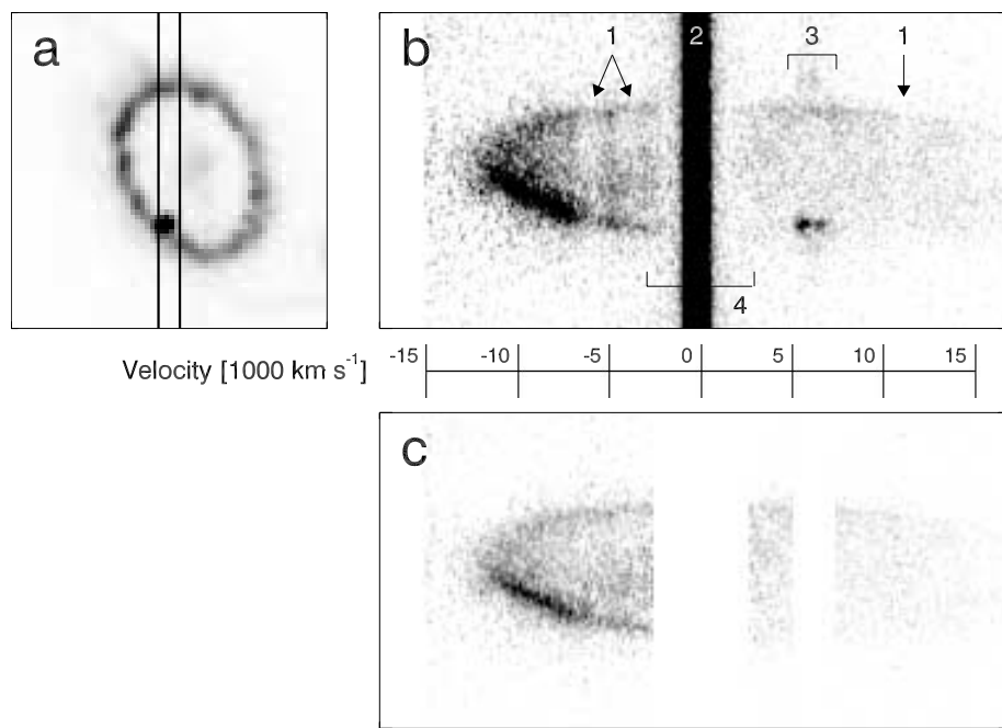
FIG. 2.—Typical Ly \alpha line profile obtained with the STIS G140L grating. (a) Location of the 0".2 slit used for this observation on the equatorial ring. The ring is shown at the same spatial scale as the line profile. (b) The spectrum in the vicinity of Ly \alpha for the L3A observation. The dispersion direction is horizontal and the spatial direction is vertical. The velocity scale is relative to the systemic velocity of SNR 1987A, v_{87A} = 287 \text{ km s}^{-1} (Meaburn et al. 1995). High-velocity Ly \alpha from the remnant appears as bright arcs and emission interior to these arcs. Numbers label the various sources of contamination of the Ly \alpha profile: (1) interstellar line absorption, (2) geocoronal Ly \alpha emission filling the slit, (3) N v \lambda\lambda 1239, 1243 emission from the ring system and spot (there are two N v spots since the line is a doublet), and (4) broad damping wings from interstellar H I absorption. (c) The “cleaned” Ly \alpha profile after the contaminants have been removed or masked out. The images in (b) and (c) are shown at different intensity stretches.
