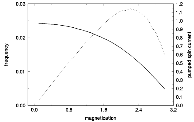
FIG. 3. The pumping frequency (solid line) and pumped spin current (dotted line) vs the magnetization of the ferromagnetic lead at which the pumped electric current is zero. For instance, when B = 1.6 and \omega = 0.02 , the system pumps out the spin current I_s = 0.96 .
