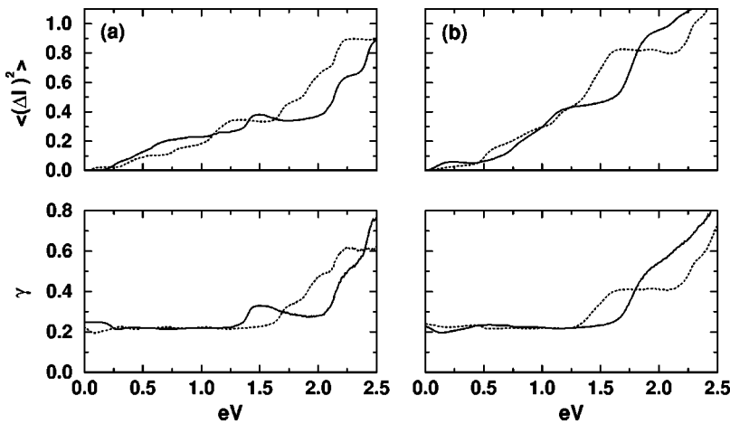
FIG. 7. Shot noise of carbon nanotube devices as obtained with the \pi -model. The top panel shows the variance of the current \langle(\Delta I)^2\rangle as a function of electron voltage, while the lower panel shows the Fano factor \gamma . Here (a) is for (5,5) tubes, and (b) for (9,0) tubes; solid line— N=10 layers; dotted line, N=11 layers, which represent on- and off-resonant devices for the respective nanotubes.
