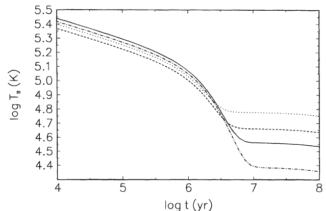
FIG. 3.—Effective surface temperature as a function of time for strange stars with B = 10^9 G for \alpha_c = 0.1 and m_s = 200 MeV (solid line), \alpha_c = 0.1 and m_s = 300 MeV (dotted line), \alpha_c = 0.4 and m_s = 200 MeV (dot-dashed line), and \alpha_c = 0.4 and m_s = 300 MeV (dashed line).
