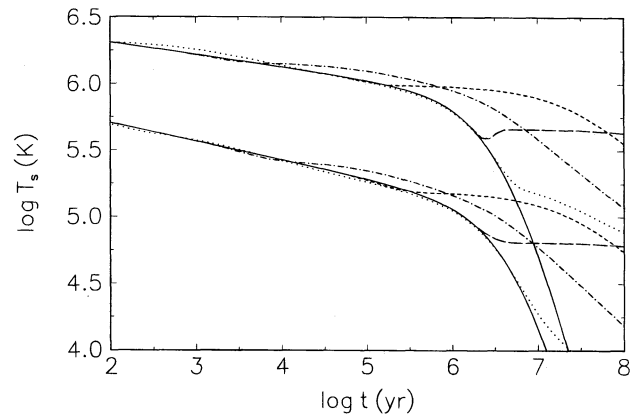
FIG. 2.—Effective surface temperature as a function of time for strange stars with \alpha_c = 0 and m_s = 300 MeV (bottom lines) and standard neutron stars (top lines). Curves are shown as in Fig. 1.
