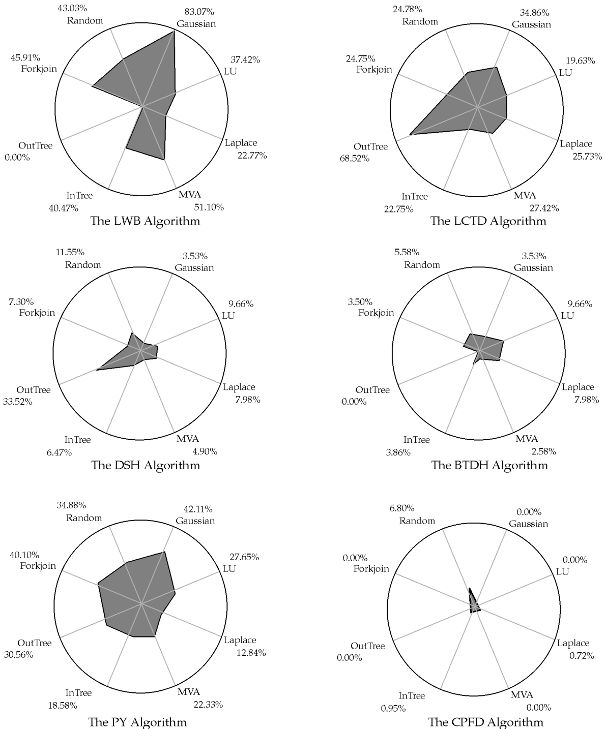
Fig. 11. Kiviatt graphs showing the average percentage degradations from the best schedule lengths of the six algorithms for various types of task graphs.
