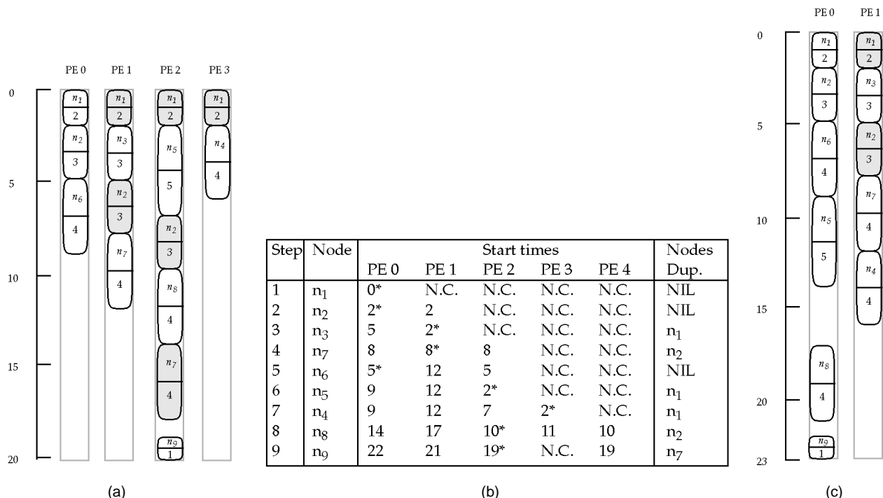
Fig. 8. (a) The schedule generated by the CPF algorithm (schedule length = 20), (b) the scheduling steps of the CPF algorithm (a node is scheduled to the processor on which the start time is marked by an asterisk and entry with "N.C." indicates the processor is not considered), (c) the schedule generated by the ECPF algorithm given only two processors (schedule length = 23).
