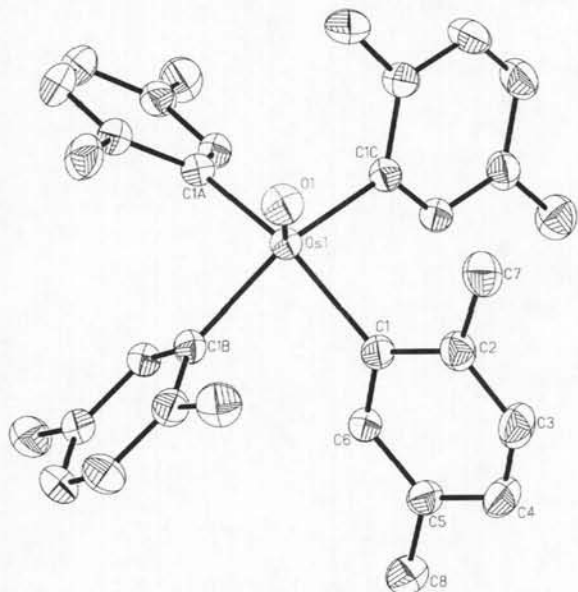
Fig. 3. Molecular structure of [\text{OsO}(\text{C}_8\text{H}_9)_4] ( 4 ). Selected bond lengths and angles are: Os(1)—O(1) 1.688(7) and Os(1)—C(1) 2.088(4) Å; O(1)—Os(1)—C(1) 110.82(12), C(1)—Os(1)—C(1B) 82.74(8), and C(1)—Os(1)—C(1A) 138.4(2)°.
