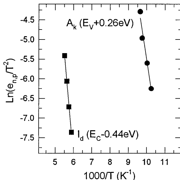
FIG. 2. Arrhenius plots of electron or hole ( e_{n,p} ) emission rates as a function of 1000/T , for deep levels corresponding to minority-carrier peak (Al-acceptor A_k ●) and majority-carrier peak (Al-induced defect I_d ■).
