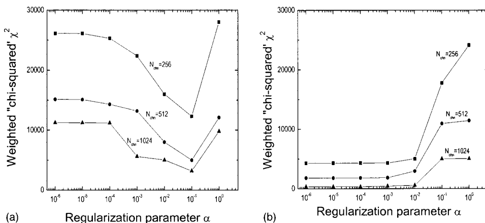
FIG. 9. Variation of the chi-squared \chi^2 of residuals plotted against the regularization parameter \alpha for synthetic CDBS spectra obtained using the 2DNGLSD algorithm; (a) with N_{\text{cts}}=10^4 and (b) with N_{\text{cts}}=10^8 . The data are shown for the different CDBS matrix sizes or N_{\text{chn}}=256 , 512, and 1024.
