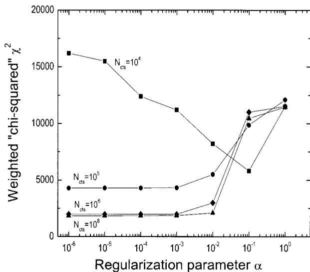
FIG. 8. Variation of the chi-squared \chi^2 of residuals plotted against the regularization parameter \alpha for synthetic CDBS spectra having N_{\text{cts}}=10^4 , 10^5 , 10^6 , and 10^8 counts, deconvoluted using the 2DNGLSD algorithm. The zeroth norm regularization was used, with N_{\text{chn}}=512 .
