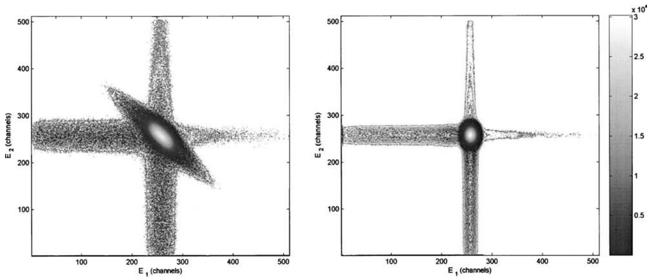
FIG. 1. (a) Experimental CDBS 2D histogram spectrum taken for polycrystalline Al metal ( N_{\text{cts}}=2 \times 10^7 ). (b) Effective CDBS 2D histogram resolution function as obtained using a ^{85}\text{Sr} source ( E_\gamma=514 keV) taken with random events (coincidence time window = 2 \mu\text{s} , N_{\text{cts}}=5 \times 10^7 ). The energy calibration for both spectra is 75 eV/channel. As can be seen, the resolution of the E_1 detector (1.2 keV) is superior to that of the E_2 detector (2.0 keV).
