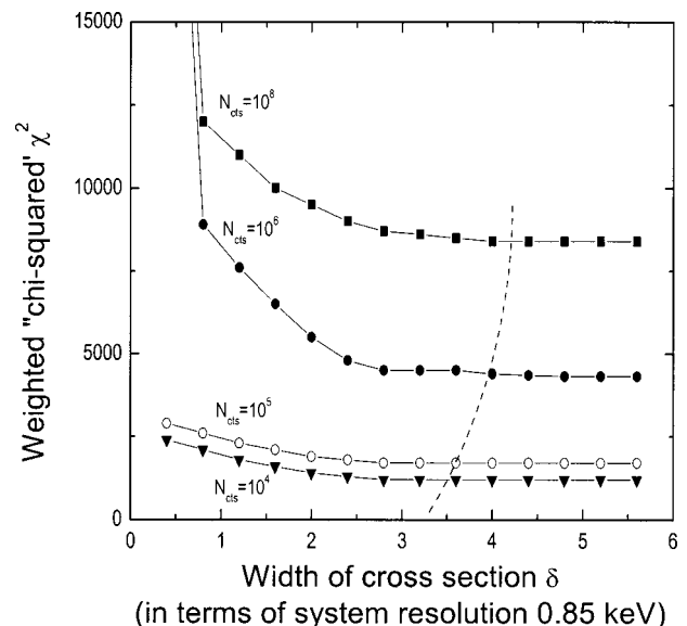
FIG. 7. Variation of summed weighted squared residuals, chi-squared, \chi^2 plotted as a function of the cutting width \delta along the CDBS diagonal for spectra having N_{cts} = 10^4, 10^5, 10^6, and 10^8 counts. The dotted line indicates the value of \delta for which \chi^2 is minimum.
