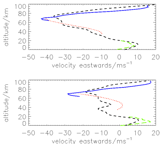
Fig. 5. Mean zonal wind recorded with the MF radar (solid blue line), falling spheres (short dashed red line) and radiosondes (long dashed green line) for January (upper panel) and February (lower panel). HWM-93 model zonal winds are shown for comparison (dashed black line). Error bars (see Figs. 3 and 4) are omitted for clarity.
