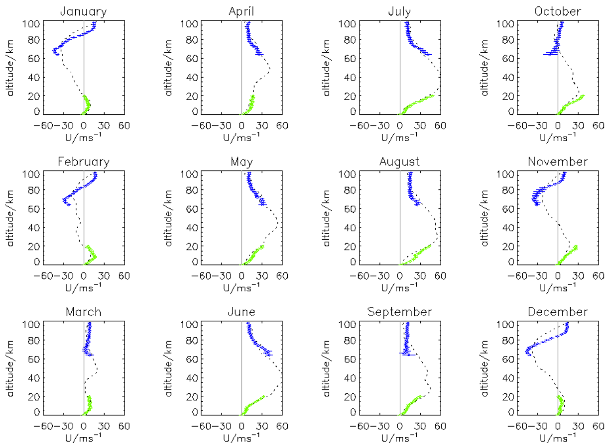
Fig. 4. As Fig. 3 but for Rothera zonal winds.
