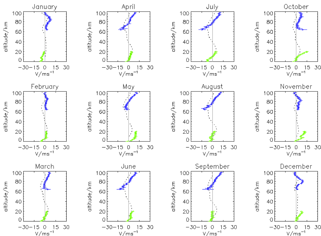
Fig. 3. Rothera monthly mean meridional winds below 100 km. Green diamonds: radiosonde data; blue diamonds MF radar winds. The error bars represent the standard error of the mean. The dotted black line is the monthly mean HWM-93 model meridional wind for Rothera.
