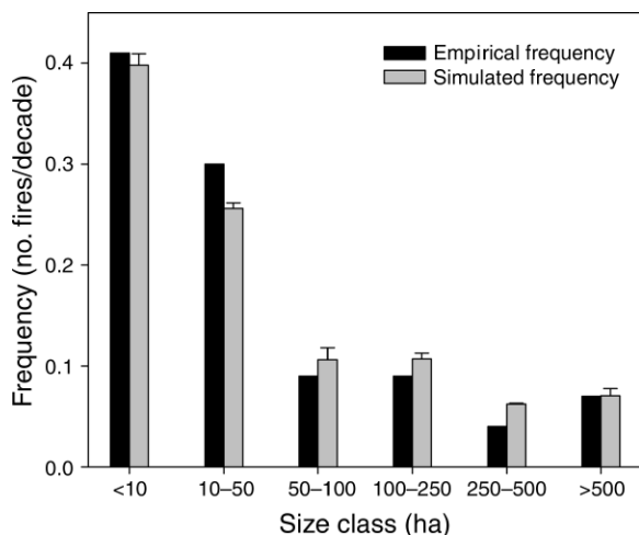
FIG. 3. Size distribution of fires ( \pm SD) in the Historic Range of Natural Variability scenario (200 simulation years).
