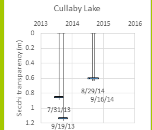
Figure 7. Cullaby Lake location, sampling sites, temperature profiles, and Secchi transparencies.
