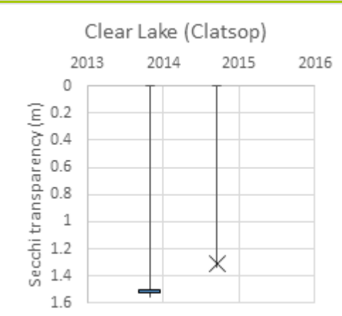
Figure 4. Clear Lake sampling sites, temperature profiles, and Secchi transparencies. X's represent measurements where the Secchi disk was visible to the bottom of the lake.
