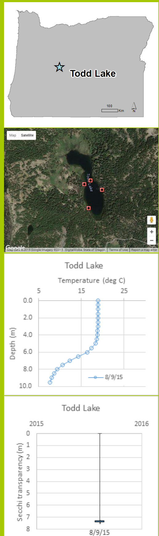
Figure 19. Todd Lake location, sampling sites, temperature profile, and Secchi transparency measurement.
