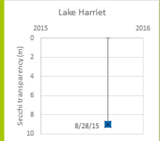
Figure 8. Lake Harriet location, sampling sites, temperature profiles, and Secchi transparency. X's represent measurements where the Secchi disk was visible to the bottom of the lake.
