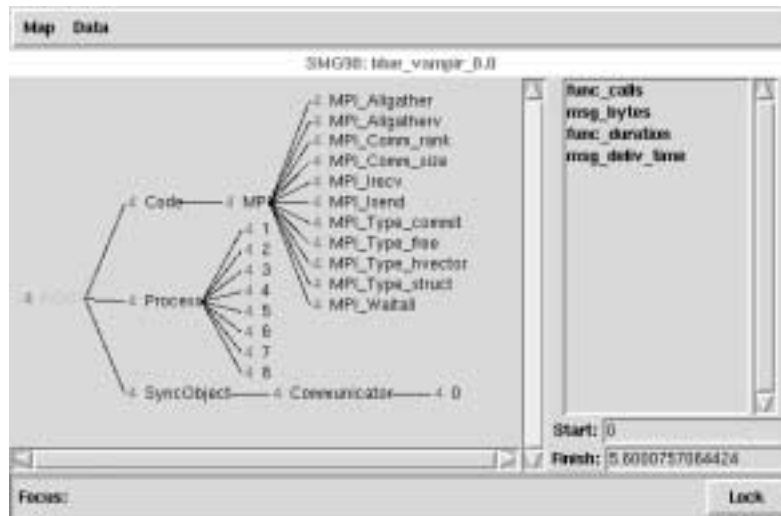
Figure 10: Vampir Tracefile
