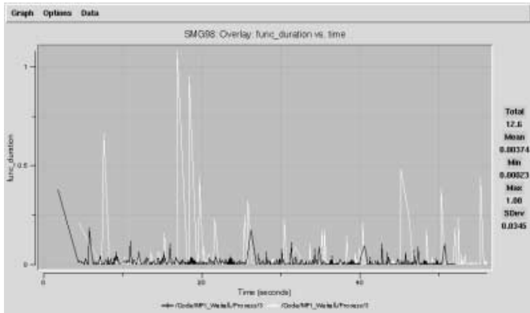
Figure 14: MPI_Waitall Times for US and IP Communication Protocols
