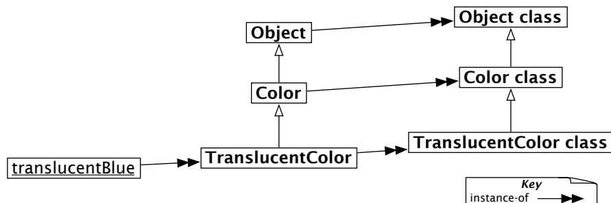
Figure 13.4: The metaclass hierarchy parallels the class hierarchy.
