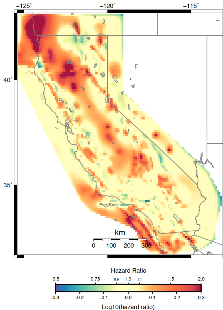
Figure C8. Map showing ratio of calculated hazard from UCERF3.2 to that from the National Seismic Hazard Map Program version of 2008 (NSHMP08); red shaded areas thus show hazard increases relative to NSHMP08, and blue areas indicate reductions. The increase in hazard in northwest California was caused by excessive slip rate placed on the Big Lagoon Fault on a block boundary in the average block model.
