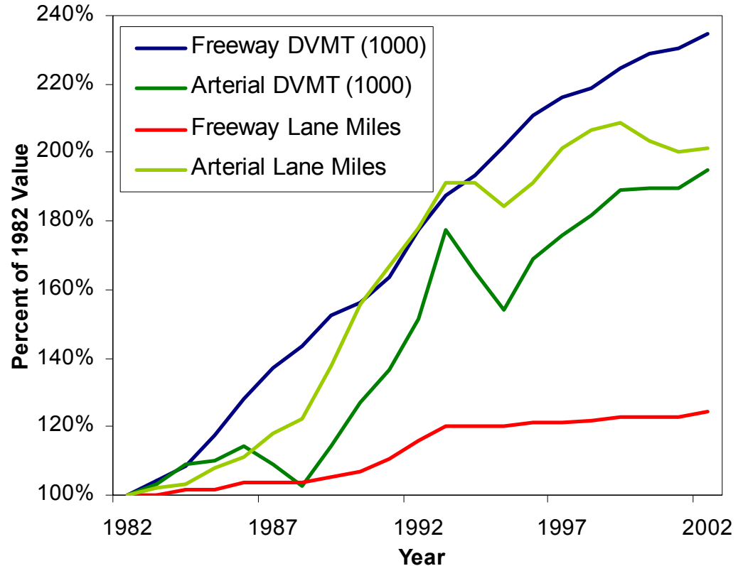
Portland Freeway and PAS VMT and Lane Miles, 1982-2002
