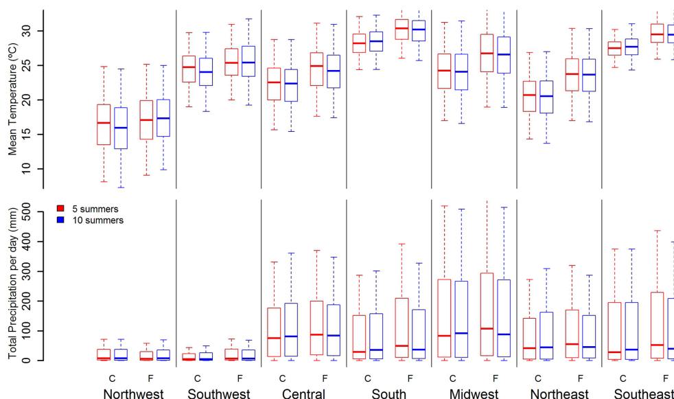
Figure 8. (Top panel) mean regional temperature for the five chosen summers (red) and ten summers (blue) of the current (C) and future (F) decades. (Bottom panel) total regional precipitation per day for the five chosen summers (red) and ten summers (blue) of the current (C) and future (F) decades. Each box-and-whisker indicates median, 5, 25, 75 and 95 % quartiles within each region.
