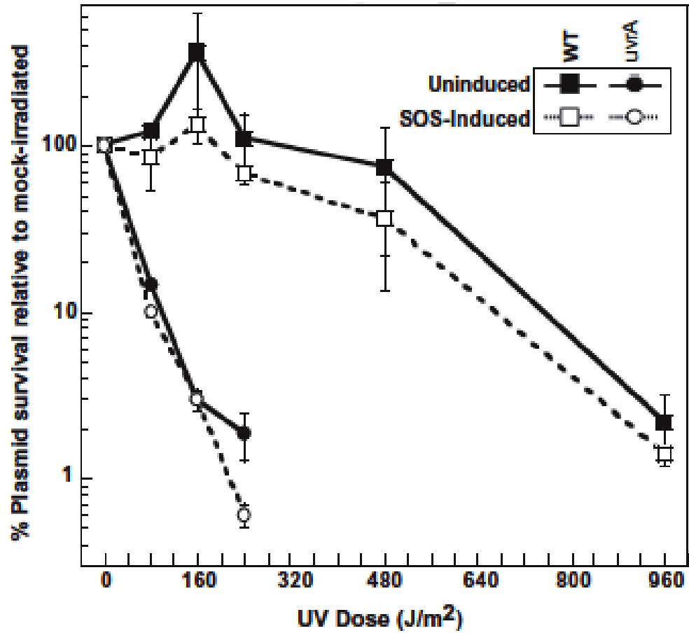
Figure 2.5. Constitutive recA expression does not enhance the survival of transforming UV-damaged plasmids. The survival of UV-irradiated plasmids following introduction into wild-type (filled squares), lexA (open squares, dotted lines), uvrA (filled circles), and uvrA lexA (open circles, dotted lines) cells is plotted relative to the survival of mock-irradiated plasmids. Plots represent an average of at least 2 experiments. Error bars represent standard error of the mean.
