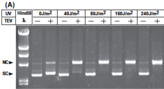
Figure 2.3. UvrA is nearly essential for the survival of transforming plasmids containing UV-induced damage. A) The formation of the predominant UV-induced lesion, the cyclobutane pyrimidine dimer (CPD), increases linearly with UV dose. The presence of lesions was determined by sensitivity to T4 Endonuclease V (TEV), which cleaves DNA at sites containing CPDs converting supercoiled plasmid (SC) to a nicked open circular form (NC). These forms are differentiated by their migration pattern following agarose-gel electrophoresis 54 . B) The survival of UV-irradiated plasmids following transformation in recA (filled bars) and uvrA (unfilled bars) mutants is plotted relative to the survival of plasmids introduced into wild-type cells at each dose. Survival was calculated as described in Figure 2.1. Plots represent an average of at least 2 independent experiments. Error bars represent standard error of the mean. C) The survival of UV-irradiated transforming plasmid is plotted relative to the survival of the mock-irradiated plasmid for wild-type (open squares), recA (open circles), uvrA (open triangles) and recA uvrA (open diamonds) at the indicated doses. The predicted (dashed line) and measured (filled squares) fraction of lesion-free plasmids in the UV-irradiated population is plotted. Measured lesion-free fractions were calculated from the amount of plasmid remaining resistant to TEV cleavage as shown in Figure 2.3A. Predicted lesion-free
