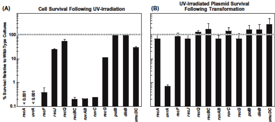
Figure 2.2. Many RecA-mediated processes that contribute to cell survival do not contribute to the survival of transforming plasmids. A) The survival of each mutant is plotted relative to the survival of wild-type cells following irradiation with 25 \text{ J/m}^2 of UV. B) The survival of UV-irradiated plasmids ( 160 \text{ J/m}^2 ) introduced into each mutant is plotted relative to the survival of plasmids introduced into wild-type cells. Data represents an average of at least 3 independent experiments. Error bars represent standard error of the mean.
