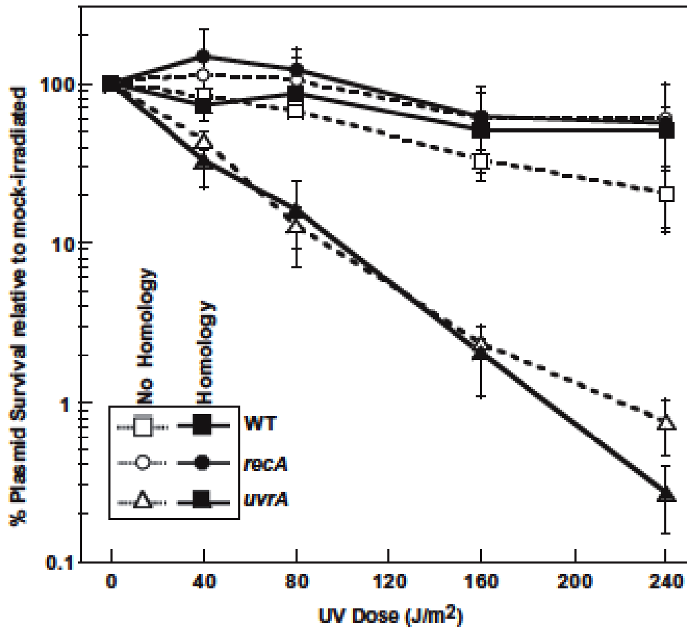
Figure 2.6. The presence of a homologous plasmid does not enhance the survival of transforming UV-damaged plasmids. The survival of UV-irradiated plasmids following introduction into wild-type (squares), recA (circles) and uvrA (triangles) cells is plotted relative to the survival of mock-irradiated plasmids at each dose. The cells either contained an endogenous homologous plasmid (filled symbols) or no homologous plasmid (open symbols, dotted lines). Plots represent an average of at least 2 experiments. Error bars represent standard error of the mean.
