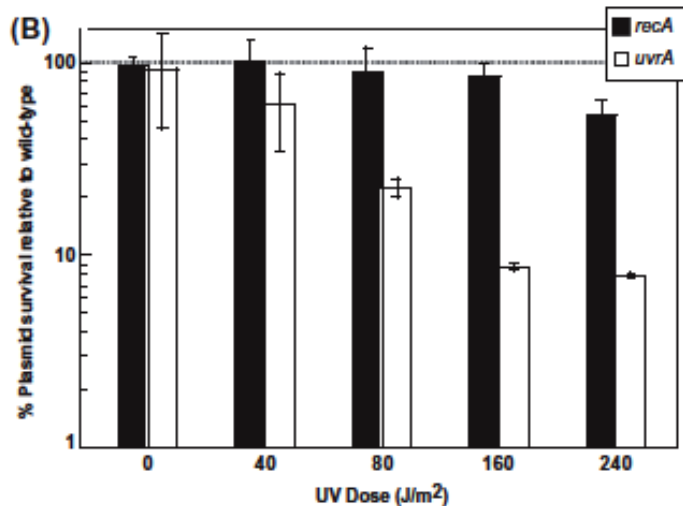
Figure 2.3. UvrA is nearly essential for the survival of transforming plasmids containing UV-induced damage. A) The formation of the predominant UV-induced lesion, the cyclobutane pyrimidine dimer (CPD), increases linearly with UV dose. The presence of lesions was determined by sensitivity to T4 Endonuclease V (TEV), which cleaves DNA at sites containing CPDs converting supercoiled plasmid (SC) to a nicked open circular form (NC). These forms are differentiated by their migration pattern following agarose-gel electrophoresis 54 . B) The survival of UV-irradiated plasmids following transformation in recA (filled bars) and uvrA (unfilled bars) mutants is plotted relative to the survival of plasmids introduced into wild-type cells at each dose. Survival was calculated as described in Figure 2.1. Plots represent an average of at least 2 independent experiments. Error bars represent standard error of the mean. C) The survival of UV-irradiated transforming plasmid is plotted relative to the survival of the mock-irradiated plasmid for wild-type (open squares), recA (open circles), uvrA (open triangles) and recA uvrA (open diamonds) at the indicated doses. The predicted (dashed line) and measured (filled squares) fraction of lesion-free plasmids in the UV-irradiated population is plotted. Measured lesion-free fractions were calculated from the amount of plasmid remaining resistant to TEV cleavage as shown in Figure 2.3A. Predicted lesion-free
