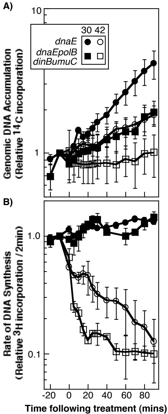
Figure B1. Following inactivation of Pol III, the rate of DNA synthesis is dependent on at least one of the damage-inducible polymerases. Cultures grown in [ 14 C]thymine at 30°C were pulse-labeled with 1 n Ci/10 n g/ml [ 3 H]thymidine for two minutes at the indicated times following mock treatment or a shift to 42°C. The amount of radioactivity incorporated into the DNA, relative to pretreated cultures is plotted. Error bars represent standard error of two experiments.
