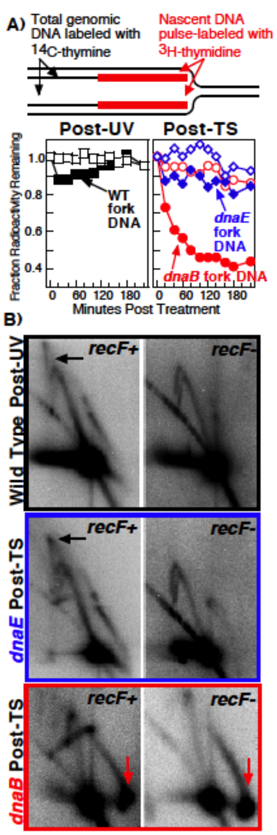
Figure 3.3. Similar to after UV, the integrity of the replication fork DNA is maintained after polymerase dissociation, and the formation of the replication fork intermediates are mediated by RecF. A) The integrity of the replication fork is maintained following arrest by UV irradiation or polymerase dissociation, but collapses after disruption of the helicase. [ ^{14}\text{C} ]-thymine prelabeled cultures were pulse-labeled with [ ^3\text{H} ] thymidine for 20 s before being filtered and placed in nonradioactive media and either UV-irradiated or shifted to 42°C as indicated. The amount of radioactivity remaining in the total genomic DNA (open symbols) and nascent DNA at the replication fork (filled symbols) is plotted over time. B) The formation and processing of the replication intermediates after polymerase dissociation are mediated by RecF, similar to UV. The formation of the abnormal intermediates that arise following helicase disruption are not dependent on RecF. Isogenic wild-type, dnaBts and dnaEts cultures containing a normal or mutated copy of the recF gene were UV-irradiated or temperature shifted and analyzed by 2D agarose gel analysis as in Figure 3.2.
