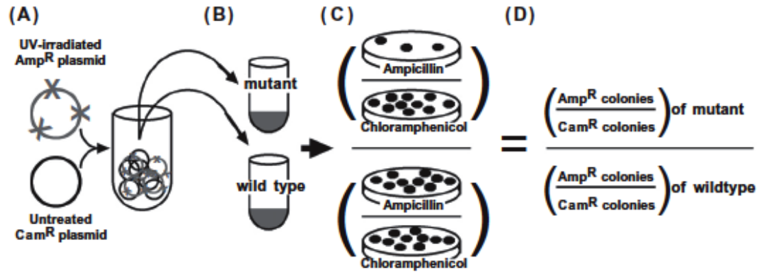
Figure 2.1. Schematic of transformation assay. A) Equal amounts of UV-damaged and untreated plasmids are mixed and used to B) transform a set of competent wild-type and mutant cells. C) The ratio of colonies formed on ampicillin plates (UV-damaged) to those formed on chloramphenicol plates (untreated) are determined for each mutant and D) normalized to the ratio observed in wild-type.
