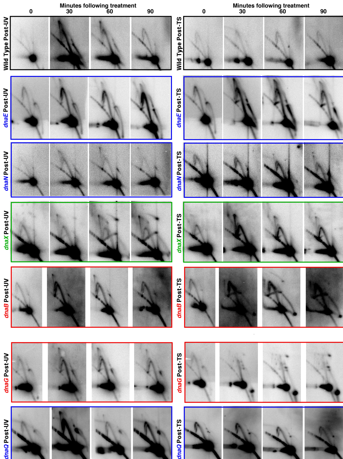
Figure 3.5. Persistence of structural intermediates that accumulate following UV exposure or inactivation by temperature shift. Aliquots each culture were taken at 0, 30, 60 and 90 minutes following treatment and subject to 2-D agarose gel analysis.
