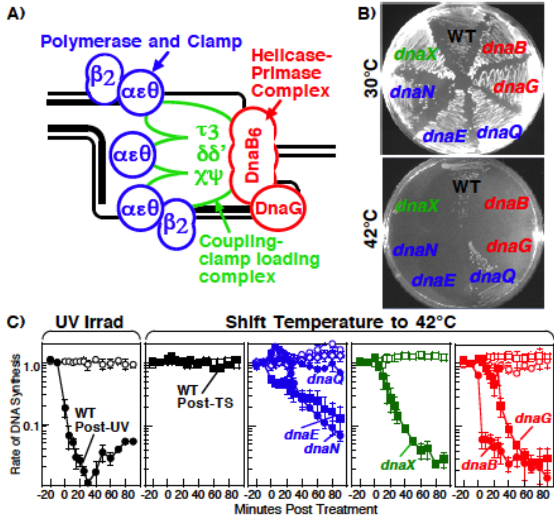
Figure 3.1. Replication is disrupted by UV-induced damage or following inactivation of the polymerase, tau complex, or helicase-primase complex. (A) A diagram of the replisome, indicating the subunits of each protein complex. (B) Thermosensitive mutants that inactivate the polymerase core, tau complex, or helicase complex are viable at 30°C but fail to grow at the restrictive temperature of 42°C following overnight incubation. (C) The rate of DNA synthesis is inhibited following UV-induced damage or inactivation of the replisome's essential subunits. Wild-type or mutant cultures, grown at 30°C were pulse-labeled with ^{14}\text{C}/10^8\text{g/ml} 3H-thymidine for two minutes at the indicated times following mock treatment (open symbols), 50 J/m ^2 UV irradiation (filled symbols), or a shift to 42°C (filled symbols). The amount of radioactivity incorporated into the DNA, relative to pretreated cultures is plotted. Error bars represent standard error of two experiments.
