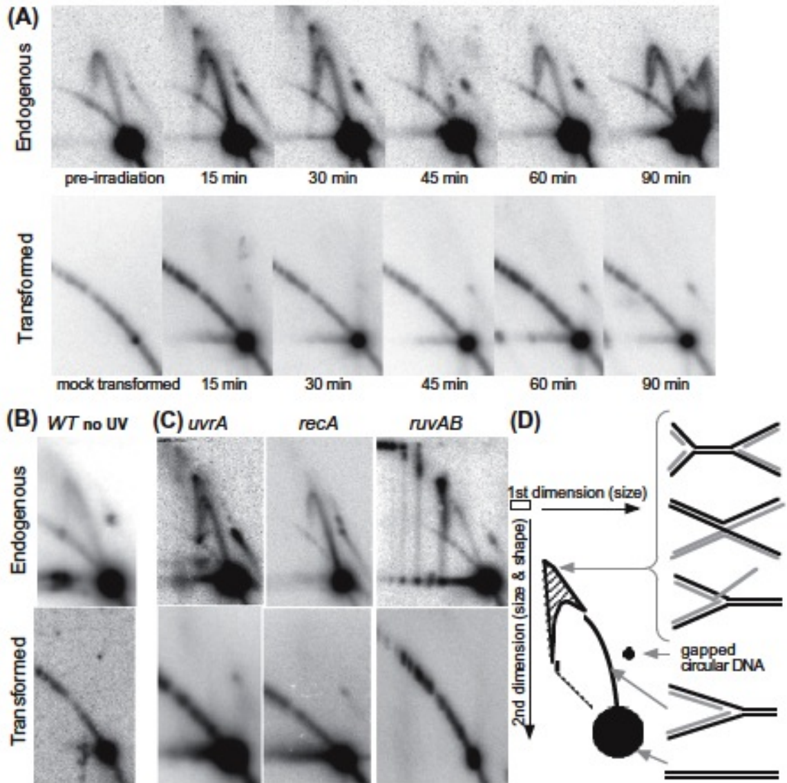
Figure 2.4. Replication- and RecA-dependent processing intermediates are not observed on newly introduced plasmids. A) Replication-associated structural intermediates observed on endogenous plasmids containing UV-induced DNA damage are not observed on plasmids following transformation. Wild-type cells containing an endogenous plasmid pBR322 were UV-irradiated with 55 \text{ J/m}^2 (top) or wild-type cells were transformed with a plasmid that was UV-irradiated with 110 \text{ J/m}^2 (bottom). Genomic DNA was then purified, digested with PvuII, and analyzed by two-dimensional agarose-gel analysis at the times indicated. B) Non-damaged plasmids also fail to generate replication intermediates when first introduced into cells. Wild-type cells containing an endogenous plasmid pBR322 were mock UV-irradiated (top) or wild-type cells were transformed with a plasmid that was mock UV-irradiated, and then analyzed as in (A) following a 60-min recovery period. C) On endogenous plasmids containing DNA damage, RecA-dependent structural intermediates persist and accumulate in uvrA and ruvAB mutants (top), but are not observed when UV-irradiated plasmids are introduced into these mutants (bottom). uvrA , recA , and ruvAB mutants were analyzed as described in (A) following UV irradiation of cultures containing an endogenous plasmid or following introduction with UV-irradiated plasmid, pBR322.
