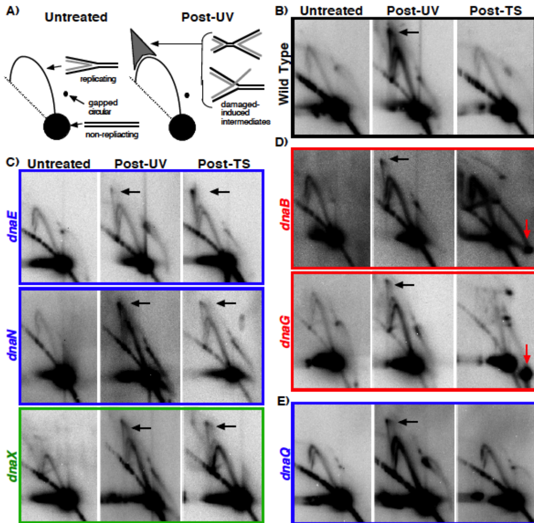
Figure 3.2. Dissociation of the DNA polymerase or \tau complex, but not the helicase complex, induces replication fork processing intermediates similar to UV-induced damage. (A) Diagram depicting the migration pattern of replicating DNA fragments and intermediates associated with processing forks disrupted by UV-induced damage in 2D agarose gels. (B) In wild-type cultures, replication fork processing intermediates are observed after disruption by UV-irradiation but not after a shift to 42°C. (C) Disruption of the polymerase core ( dnaEts ), processivity factor ( dnaNts ) or tau ( dnaXts ) is sufficient to induce replication fork processing similar to that seen after UV-induced damage. (D) Abnormal intermediates, distinct from any of those associated with processing UV-induced damage, arise after disruption of the helicase ( dnaBts ), or primase ( dnaGts ). (E) No atypical intermediates are observed following disruption of the nonessential proofreading subunit of the DNA polymerase ( dnaQts ). Strains containing plasmid pBR322 were UV-irradiated with 50 J/m 2 or filtered and placed in pre-warmed media at 42°C. Genomic and plasmid DNA was then purified, digested with PvuII, and analyzed by 2D agarose-gel analysis 15 and 90 min following UV-irradiation or temperature shift, respectively.
