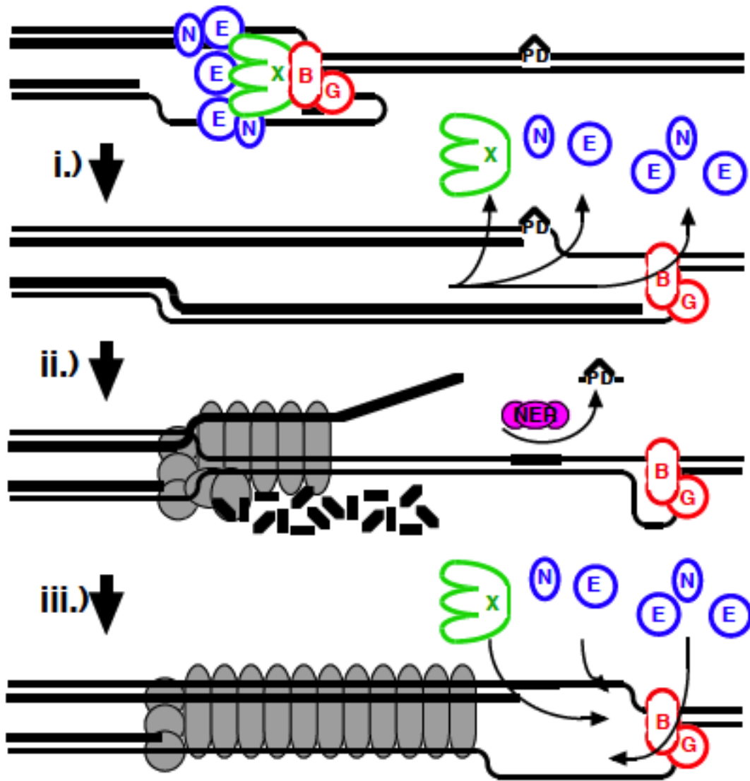
Figure 3.4. Model of Replisome at UV-induced damage. Upon encountering an arresting lesion (i), DNA synthesis becomes uncoupled and the polymerases transiently dissociate. (ii) This serves as a signal to initiate the replication fork DNA processing by the RecF pathway gene products (gray circles) allowing repair enzymes (NER) or translesion polymerases (not shown) to access the lesion. (iii) The helicase-primase complex remains bound to the template DNA and serves to maintain the licensing and integrity of the replication fork, directing replisome re-assembly to the correct location once the lesion has been processed.
