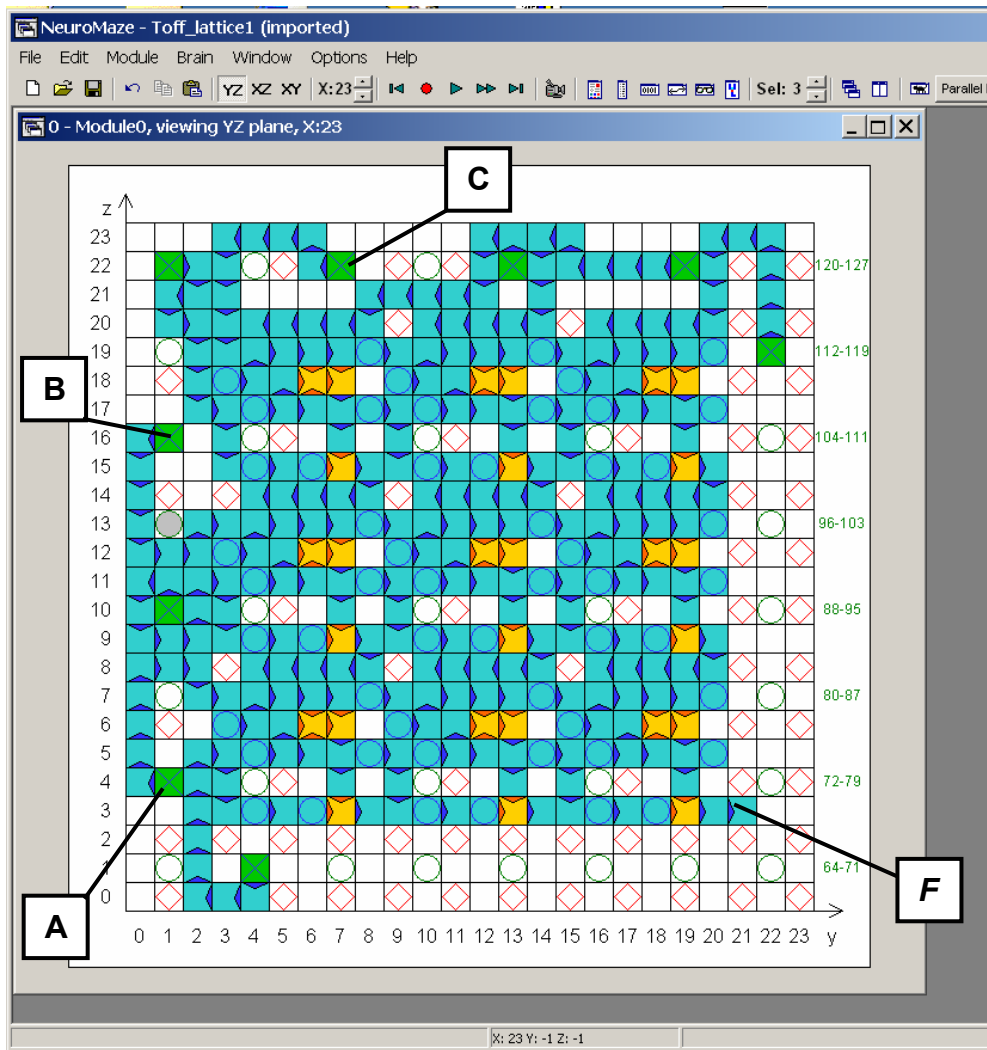
Figure 11. Davio lattice's upper layer in the NeuroMaze's worksheet. For the clock t it returns F(A_{t-3-18+8}, B_{t-4-18+8}, C_{t-5-18+8})
