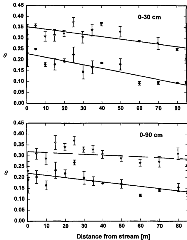
Fig. 2. Soil moisture response ranges: from drought (11 November, 1991; \circ -) through 24.3 cm precipitation recharge (2 December, 1991; \bullet -). Each point is a mean of 3 measurements. Least squares regressions of soil moisture content on distance along hillslope in the shallow layer showed significant ( p < .05 ) gradients before and after recharge. Regressions in the deeper layer showed a significant gradient during drought, but not after recharge.
