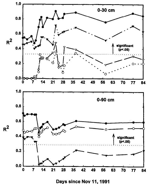
Fig. 3. Squared partial correlations for physiographic variables vs. soil moisture content during the measurement period. Physiographic variables shown are: topographic index ( \bullet -), soil storage index ( \circ -), and organic matter index ( \nabla -). Also shown are adjusted r^2 values for multiple regressions of physiographic variables on soil moisture ( \bullet -); only those variables that were significant in partial F tests ( p < .05 ) were included.
