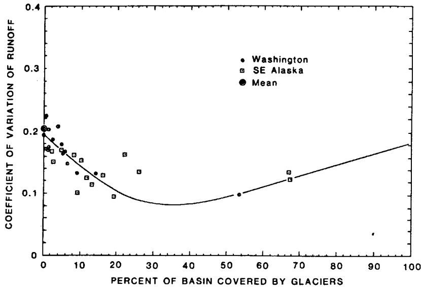
Fig. 5. Coefficient of variation of annual specific runoff values versus the fraction of the drainage basin glaciated. Circles are Washington stations; squares are Alaska sites. The mean value for unglacierized basins is indicated by the double circle. The solid line is based on (7), in which the two basins are Salix (1812) and South Cascade (1811).
