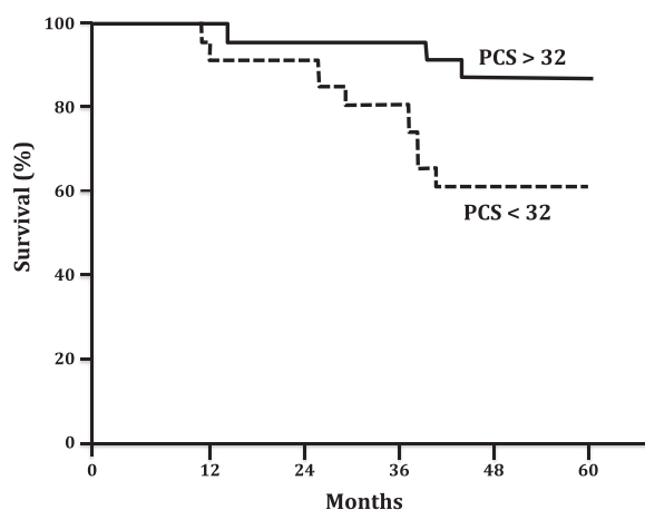
Figure 2 Kaplan Meier survival rates according baseline SF-36 Physical Component Score (PCS). Log rank test, p = 0.04 .
