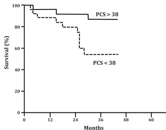
Figure 3 Kaplan Meier survival rates according SF-36 Physical Component Score (PCS) after 16 weeks of specific PAH therapy. Log rank test, p = 0.016 .
