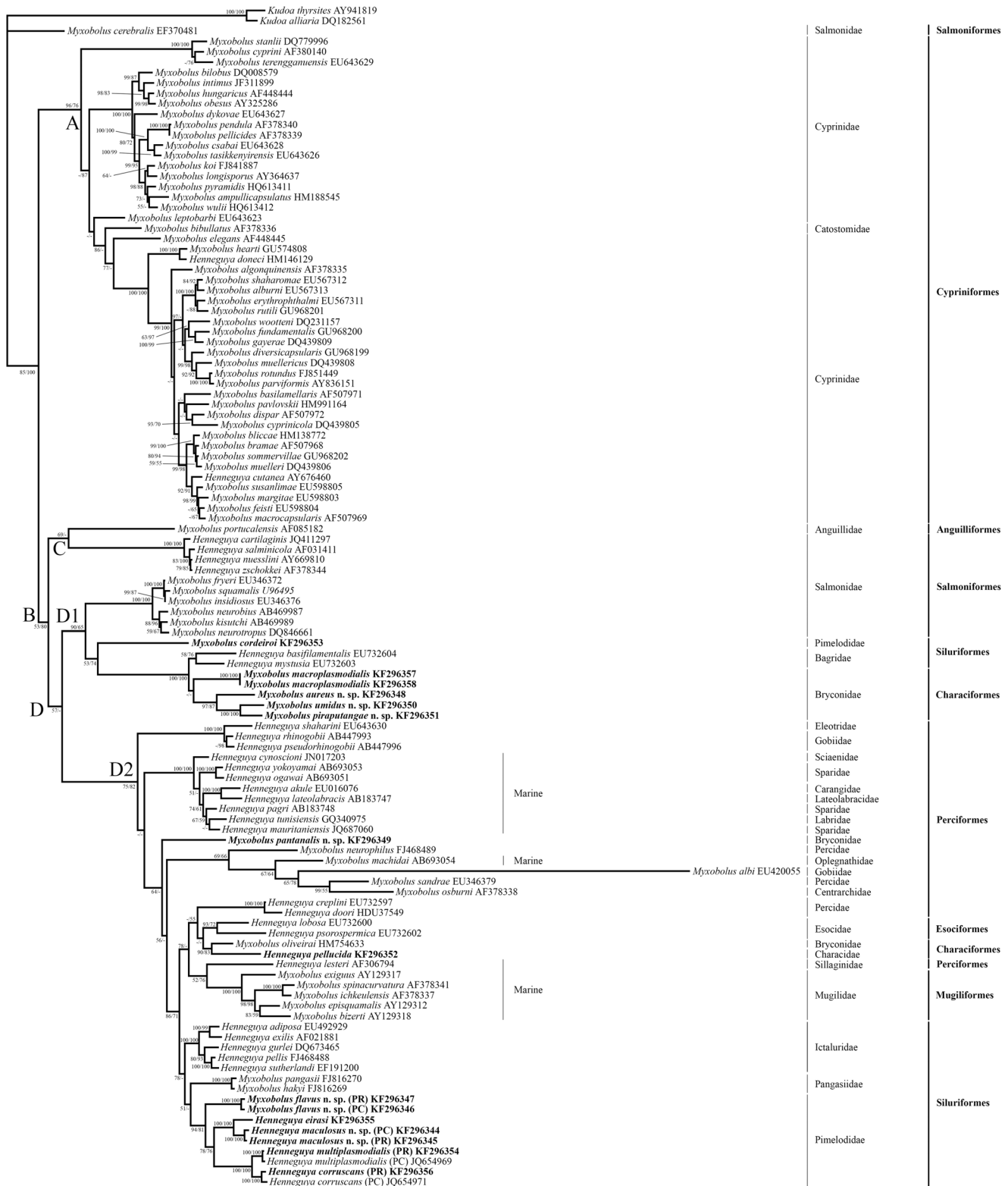
Figure 3. Maximum likelihood phylogenetic tree based on partial 18 S rDNA sequences. The bootstrap support values at branching points are listed as maximum likelihood/maximum parsimony. GenBank accession numbers are given following the name of the species. PW = Pantanal wetland; MG = Mogi Guaçu River; PC = Pseudoplatystoma corruscans ; PR = Pseudoplatystoma reticulatum . doi:10.1371/journal.pone.0073713.g003
