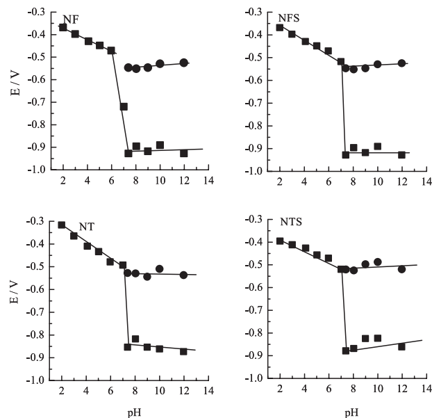
Figure 4. Potential peaks values vs. pH values. (■) E_{c,p1} values; (●) E_{c,p2R} values. [Compound] = 0.5 mmol L -1 , v = 0.10 V s -1 .
