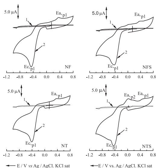
Figure 2. Cyclic voltammograms recorded at pH 4.02. (1) Blank; (2) compound. [Compound] = 0.5 mmol L -1 ; v = 0.1 V s -1 ; E_{\text{initial}} = 0.0 V, E_{\lambda,1} = -1.0 V, E_{\lambda,2} = +0.80 V, E_{\text{final}} = 0.0 V.
