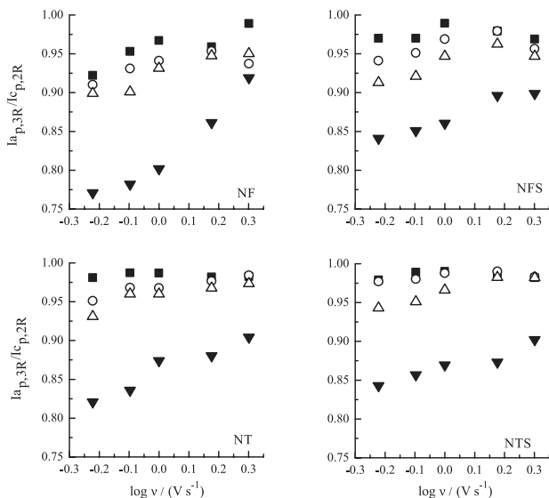
Figure 7. Relationship between I_{p,3R}/I_{c,p,2R} ratio vs. \log v . [Compound] = 0.5 mmol L -1 ; pH values: 8.03 ( \nabla ); 9.02( \Delta ); 10.01 ( \circ ); 12.01( \blacksquare ).
