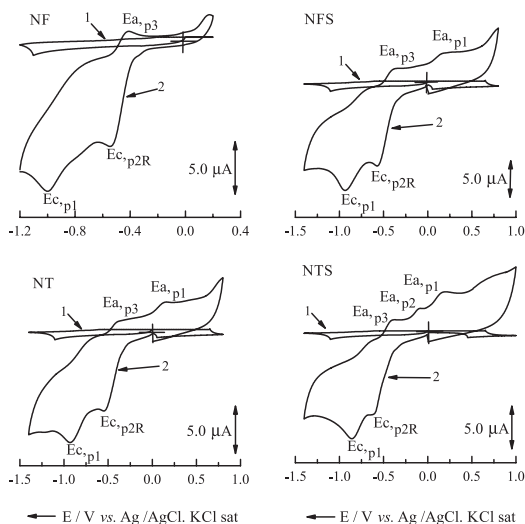
Figure 3. Cyclic voltammograms recorded at pH 7.41. (1) Blank; (2) compound. [Compound] = 0.5 mmol L -1 ; v = 0.1 V s -1 ; E_{initial} = 0.0 V, E_{\lambda 1} = -1.2 V < E_{\lambda} < -1.5 V, E_{\lambda 2} = +1.0 V; E_{final} = 0.0 V.
