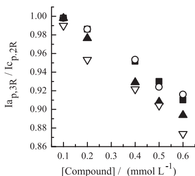
Figure 8. Effect of the compound concentration on I_{p,3R}/I_{c,p,2R} ratio at pH 10.01. ( \blacksquare ) NF; ( \circ ) NFS; ( \blacktriangle ) NT; ( \nabla ) NTS.
