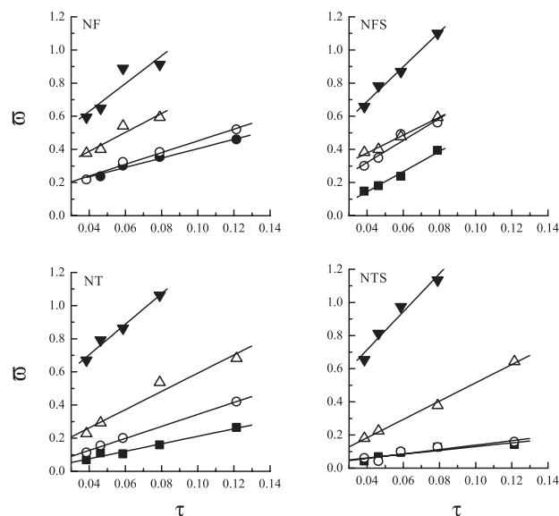
Figure 9. Plots of the kinetic parameters: \omega vs. \tau . [Compound] = 0.50 mmol L -1 . pH values: 8.02 ( \blacktriangledown ); 9.02 ( \Delta ); 10.01 ( \circ ); 12.01 ( \blacksquare ).
