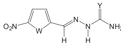
Figure 1. Chemical structure of nitrofurazone (NF, W = O; Y = O) and its analogues: NFS (5-nitro-2-furfurylidene thiosemicarbazone, W = O; Y = S); NT (5-nitro-2-thiophene semicarbazone, W = S; Y = O) and NTS (5-nitro-2-thiophene thiosemicarbazone, W = S; Y = S).
