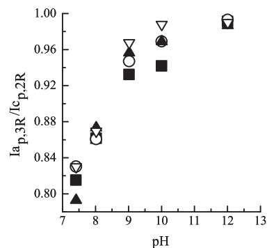
Figure 6. Effect of pH values on I_{a,p3R}/I_{c,p2R} . (■) NF; (○) NFS; (▲) NT; (▽) NTS. [Compound] = 0.50 mmol L -1 .
