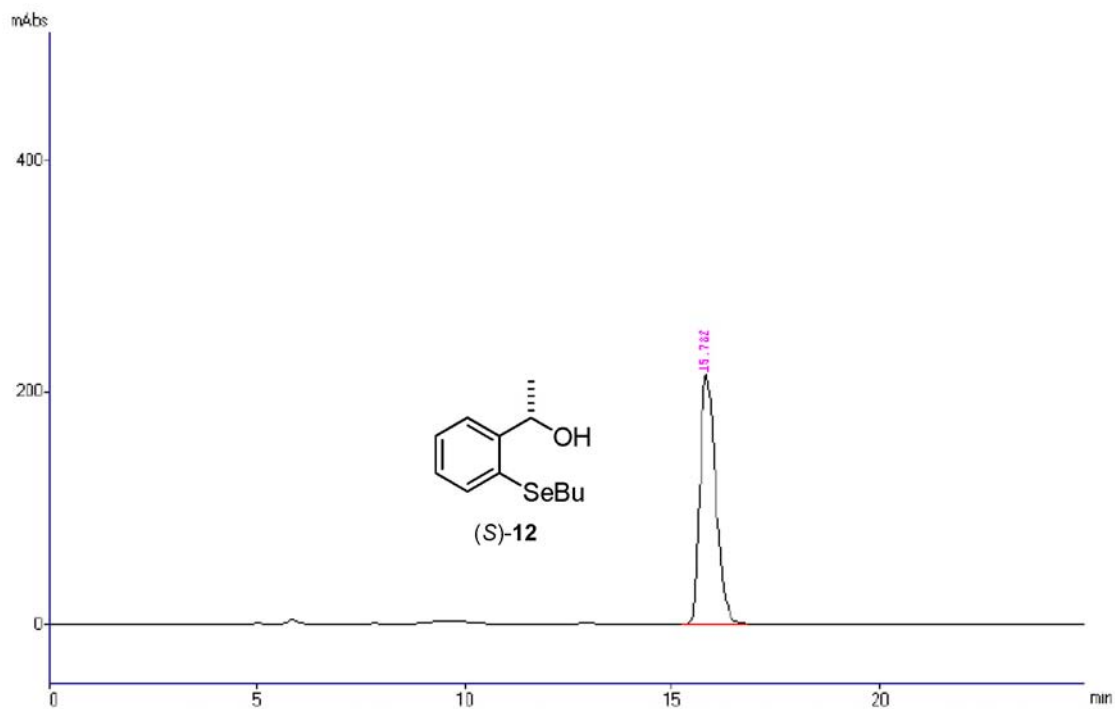
Figure S57. (S)-1-(2-(butylselanyl)phenyl)ethanol ( 12 ): Isolated yield = 45%; Enantiomeric excess > 99%; [\alpha]_D^{22} = -23.9 ( c = 0.78 ; \text{CHCl}_3 ). HPLC condition: Chiralcel ® OJ-H column, n -hexane/ i -PrOH (99:1), 1.0 mL min -1 , 254 nm UV detector, t_R = 15.8 min.
