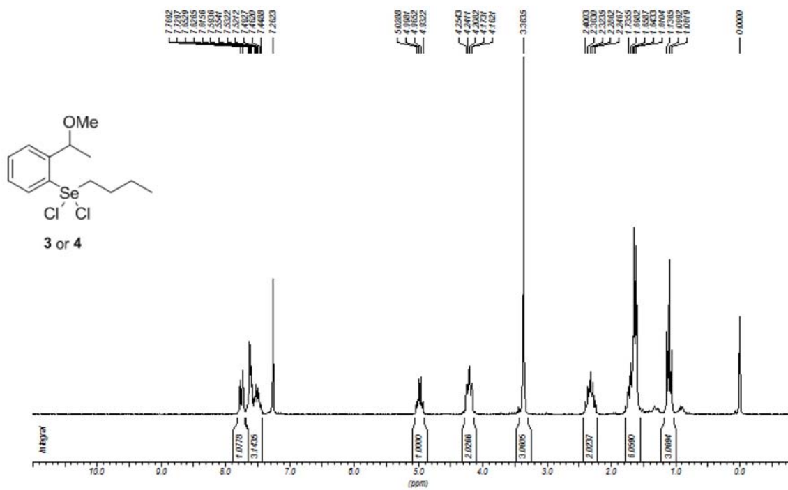
Figure S18. 1 H NMR (200 MHz, CDCl 3 ) spectrum of selenane (3 or 4).
