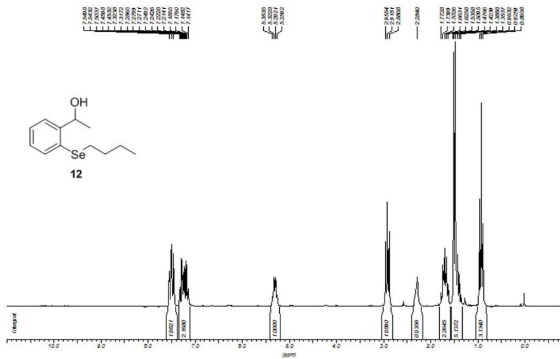
Figure S5. 1 H NMR (200 MHz, CDCl 3 ) spectrum of 1-(2-(butylselanyl)phenyl)ethanol ( 12 ).
