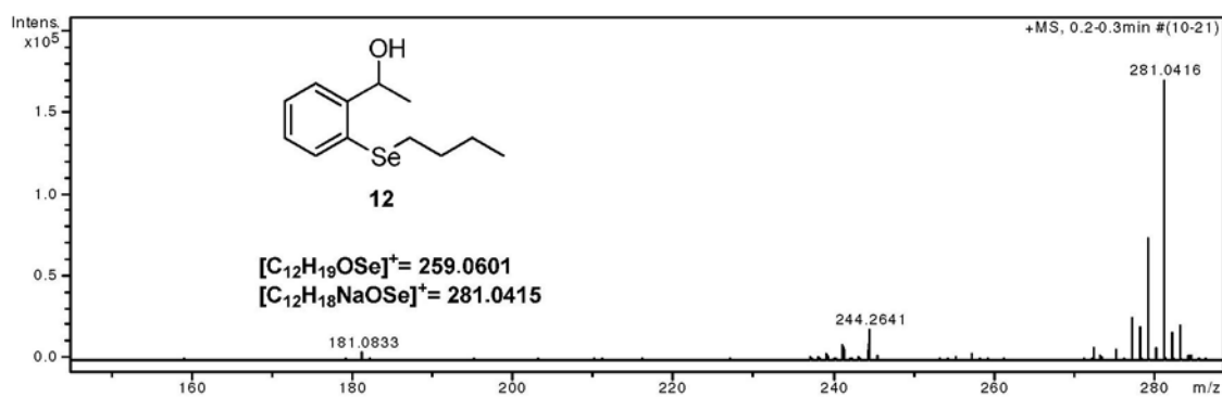
Figure S8. High resolution mass spectrum (ESI) of 1-(2-(butylselanyl)phenyl)ethanol ( 12 ).
