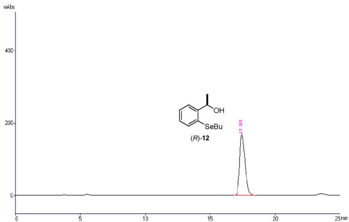
Figure S58. (R)-1-(2-(butylselanyl)phenyl)ethanol ( 12 ): Isolated yield = 45%; Enantiomeric excess > 99%; [\alpha]_D^{22} = +24.1 ( c = 0.80 ; \text{CHCl}_3 ). HPLC condition: Chiralcel ® OJ-H column, n -hexane/ i -PrOH (99:1), 1.0 mL min -1 , 254 nm UV detector, t_R = 17.3 min.
