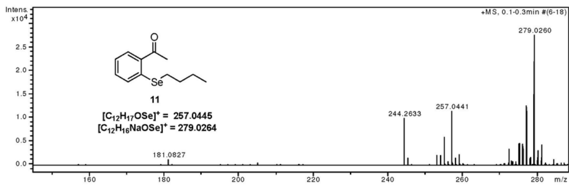
Figure S4. High resolution mass spectrum (ESI) of 1-(2-(butylselanyl)phenyl)ethanone ( 11 ).
