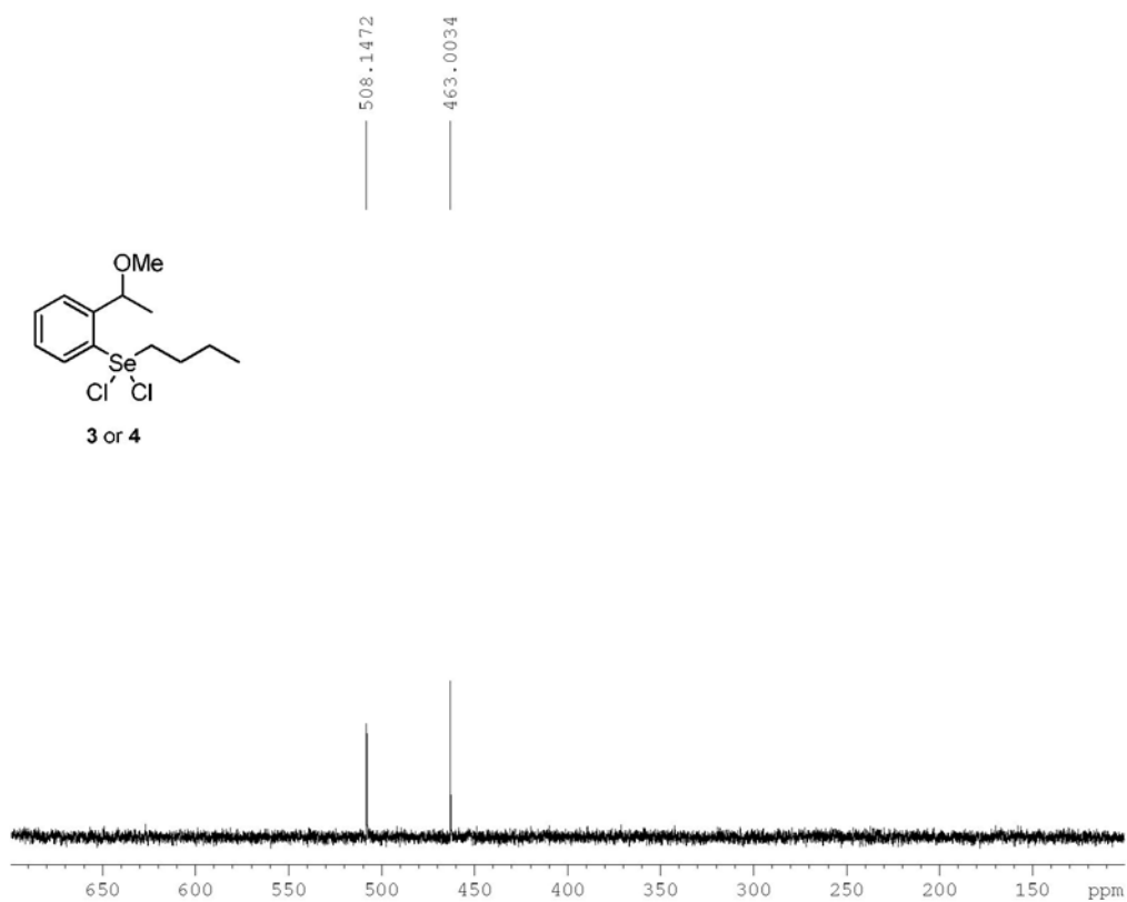
Figure S20. 77 Se NMR (57.24 MHz, CDCl 3 ) spectrum of selenane (3 or 4).
