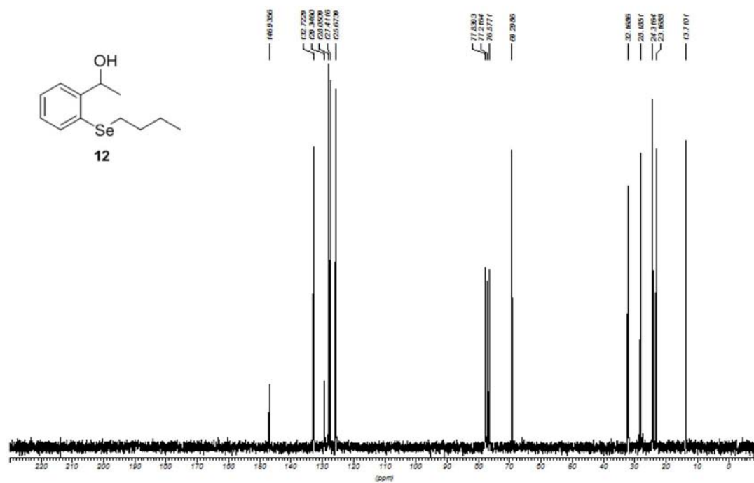
Figure S6. 13 C NMR (50 MHz, CDCl 3 ) spectrum of 1-(2-(butylselanyl)phenyl)ethanol ( 12 ).
