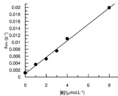
Figure S55. Enzyme kinetic for cathepsin S using selenane 6 as inhibitor.
