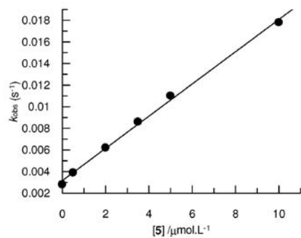
Figure S54. Enzyme kinetic for cathepsin S using selenane 5 as inhibitor.
