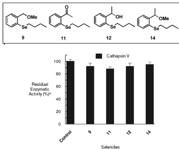
Figure S42. Inhibition profile for cathepsin V using selenides 9, 11, 12 and 14 ( 1 \mu\text{mol L}^{-1} ). Conditions: Cathepsin V in sodium acetate buffer ( 50 \text{ mmol L}^{-1} ; pH 5.5) containing EDTA ( 2.5 \text{ mmol L}^{-1} ). a Average of three determinations.
