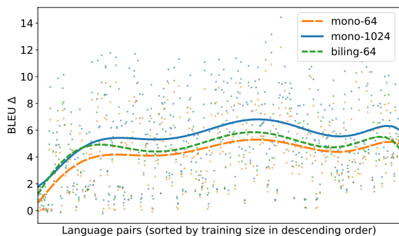
Figure 2: Comparison of bilingual adapters and monolingual adapters on the TED test sets in the adaptation setting, over 380 language pairs (sorted by available data). The y-axis shows the absolute BLEU differences with the parent model (trained on English-centric data only). The trendlines are obtained by interpolating a polynomial of degree 7 over the individual points.
