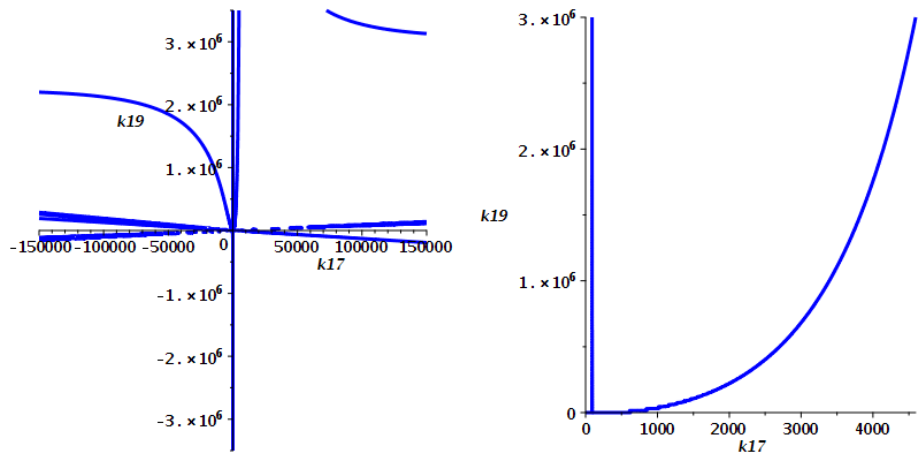
Figure 15: Numerical plot of the graph of polynomial (27) on larger ranges.
