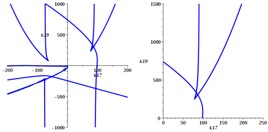
Figure 14: Numerical plot of the graph of polynomial (27) on smaller ranges.
