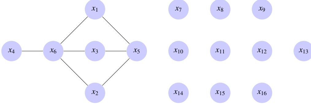
Figure 6: The graph for (28) produced according to the techniques set out in Section 5. Despite being a larger system the minimum vertex cover \{x_5, x_6\} is still small. All other variables form a maximum independent set, which can be eliminated with linear methods.
