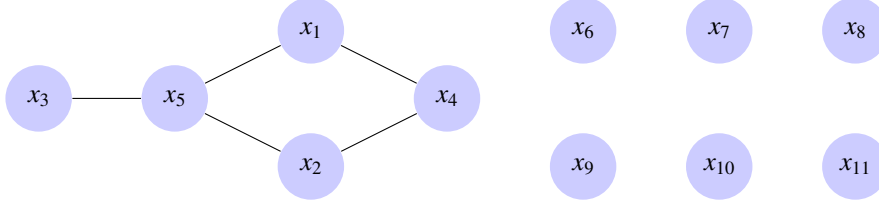
Figure 3: The graph for \overline{(1)} is loosely connected. Its minimum vertex cover \{x_4, x_5\} is small. All other variables form a maximum independent set, which can be eliminated with linear methods.
