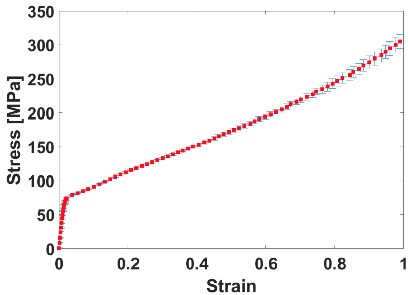
Figure 3.2 The mechanical properties of pristine PET films ( 125\ \mu\text{m} ) for five samples under uniaxial tensile tests.
