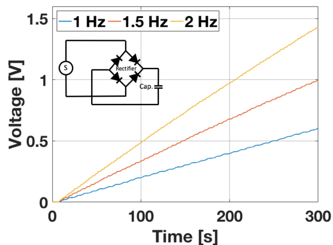
Figure 4.21 The charging of a capacitor ( 10\ \mu\text{F} ) from the rectified voltage output of the sensor under 15% strain. The inset is the circuit diagram of the energy harvesting and storage system.
