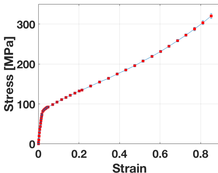
Figure 5.2 The stress-strain curves of pristine PET films ( 125 \mu\text{m} ) for five samples under uniaxial tensile tests.
