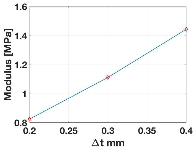
Figure 5.6 The effective modulus of the non-uniform Kirigami structures with the slit gap increment of 0.2 mm, 0.3 mm, to 0.4 mm respectively based on numerical simulations.
