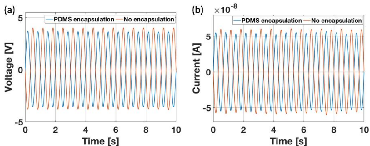
Figure 4.15 The comparisons of (a) the open-circuit voltage and (b) short-circuit current versus time before and after PDMS encapsulation at 1.5 Hz and 10% strain.
