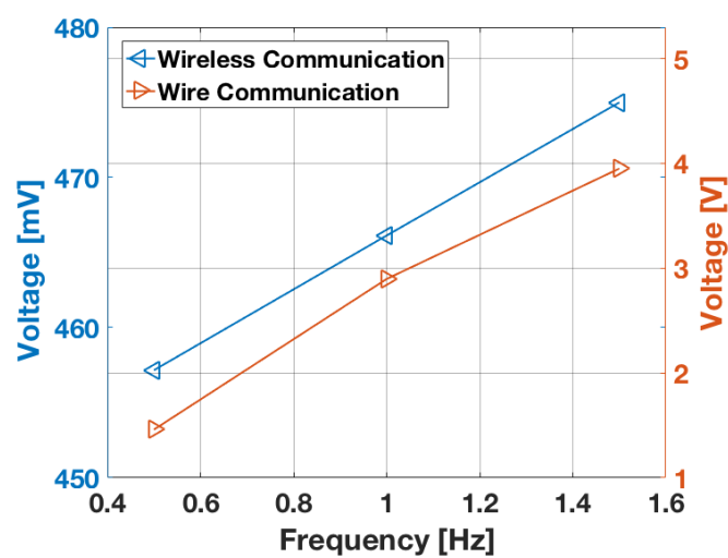
Figure 4.43 The comparative study of the sensing system under wire and wireless measuring ways with sine-shape inputs.
