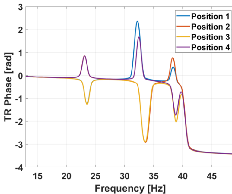
Figure 6.8 The phase of structural transmissibility in four cantilever beams for the 3D buckled structure without Kirigami cuts
