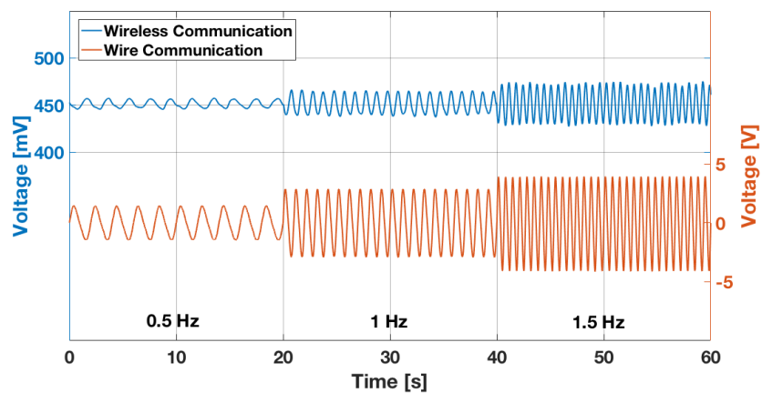
Figure 4.42 The comparative results between the wire and wireless measurement methods with sine-shape input under 4.0 kPa and three frequencies: 0.5 Hz, 1.0 Hz, and 1.5 Hz on air-driven platform.
