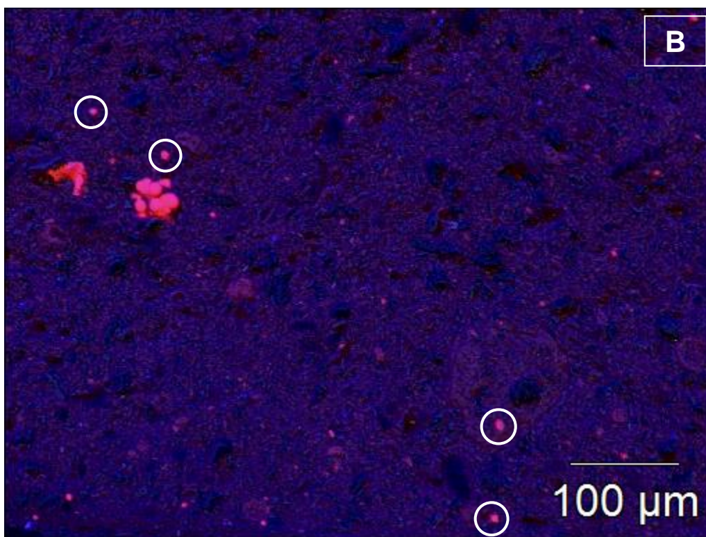
Figure 19 - Figure 19A is an SEM EDS map of iron in the A horizon of the Chenqi soils collected in 2016. White circles have been used to highlight examples of iron presence within the sample. Figure 19B is the SEM map of iron from Figure 19A with the map of phosphorus from Figure 17 overlain; this allows for the identification of iron-bound phosphorus species within the A horizon sample.
