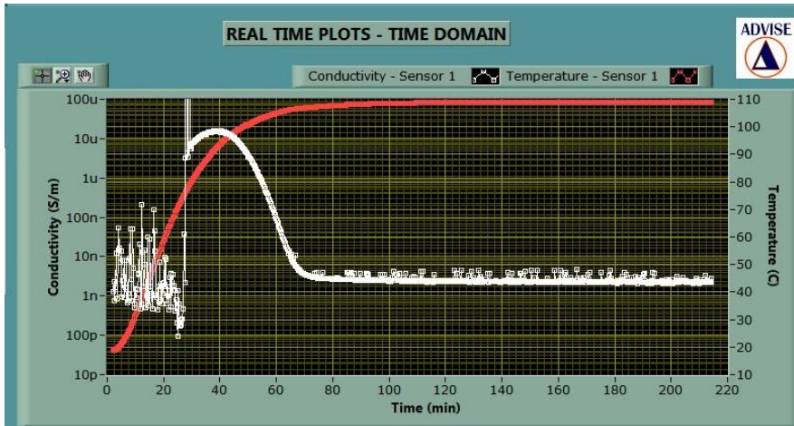
(a) Plot of conductivity and temperature versus time. The signal is noisy until the resin flows onto the sensor. Then conductivity increases with temperature until the cure begins. It appears that the cure ends at 80 minutes, but this is not the case. Note that conductivity is 1/\text{resistivity} .
