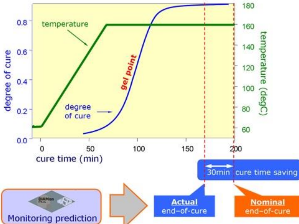
The cure cycle savings amount up to 30% of the total time (including the cooling stage), which results to significant energy savings and increased utilisation of the manufacturing tools.
