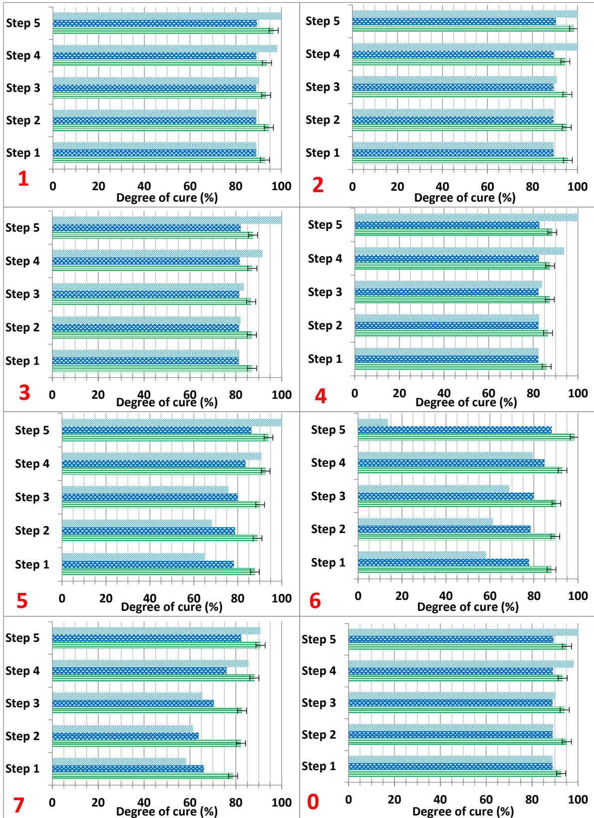
Figure 5.31: Comparison of Degree of Cure by DSC (green), Raven simulation based on thermocouple data (Sim_data) (darker blue) and Raven simulation based on theoretical cure cycle (Sim) (lighter blue).
