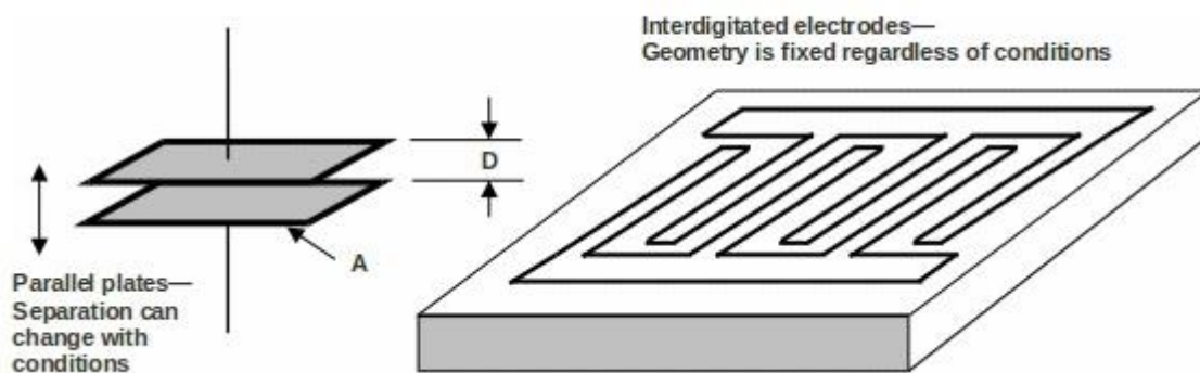
Figure: Parallel plate and interdigitated sensors, reproduced from Lambient theory guide.
