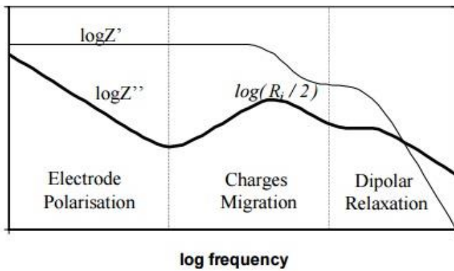
Figure 2.15: Illustration of \log Z' and \log Z'' versus \log frequency, 3 zones of the cure. Reproduced from [88].
