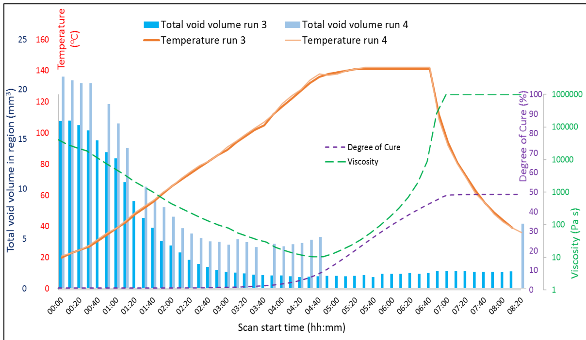
Figure 4.25: Defect evolution and resin behaviour, ply drop gap with hold at \sim 140^{\circ}\text{C} . Resin behaviour calculated from the model of Kratz et al. [43]
