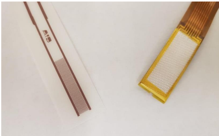
Figure 5.10: A GIA electrode (left) with a Netzsch Kapton substrate electrode (right), as used with the Advise DETA cure monitoring system. The Kapton substrate electrode is approximately 1cm wide. The interdigitated electrodes are visible on the GIA electrode, but hidden under a glass fibre veil on the Kapton electrode. The veil prevents the electrode shorting on conductive material such as carbon fibres.
