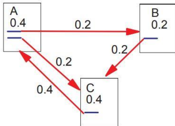
Figure 3.5: Illustration of a simplified PageRank calculation, reproduced from [194]
