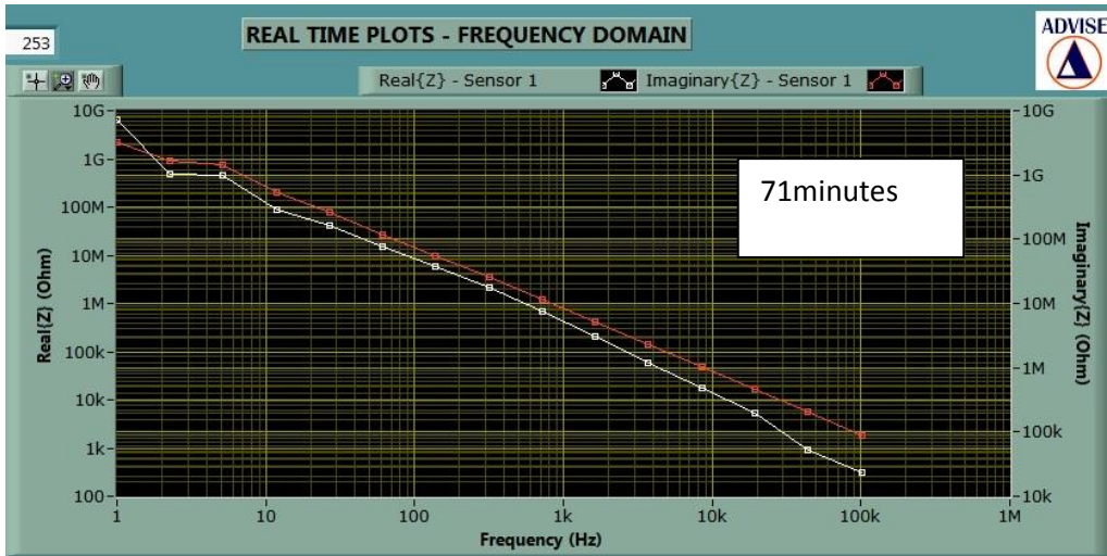
(b) Plots of Z' and Z'' at timesteps during the cure. The peak of Z'' moves beyond the equipment range, so we cannot be sure when the cure has actually completed. Compare to figure 8 for more information.
