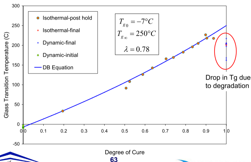
Figure 2.3: NCAMP model for 8552 resin, with parameters for DiBenedetto equation. Reproduced from [23]
