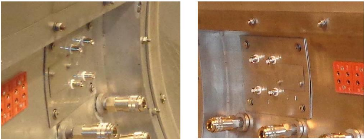
Figure y, Modifications to an existing autoclave, http://www.advise-deta.com/
