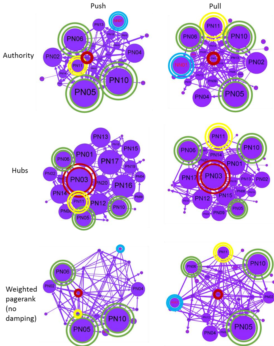
Figure 3.7: Push and pull networks for Company 8, with nodes sized by Authority, Hubs and Weighted PageRank (no damping). Nodes highlighted in green represent known senior figures at the company. Person PN03 is highlighted in red, person PN11 in yellow and person NN01 in blue. Non-participants labelled in red.
