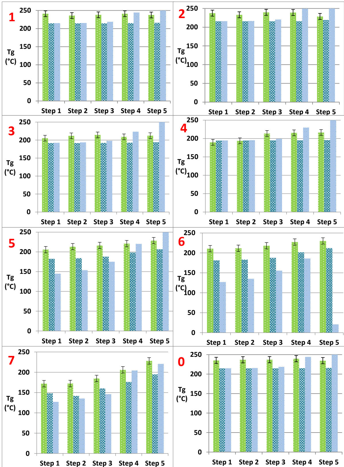
Figure 5.30: Comparison of T_g by DMA tan \delta peak (green), Raven simulation based on thermocouple data (Sim_data)(darker blue) and Raven simulation based on theoretical cure cycle (Sim) (lighter blue).
