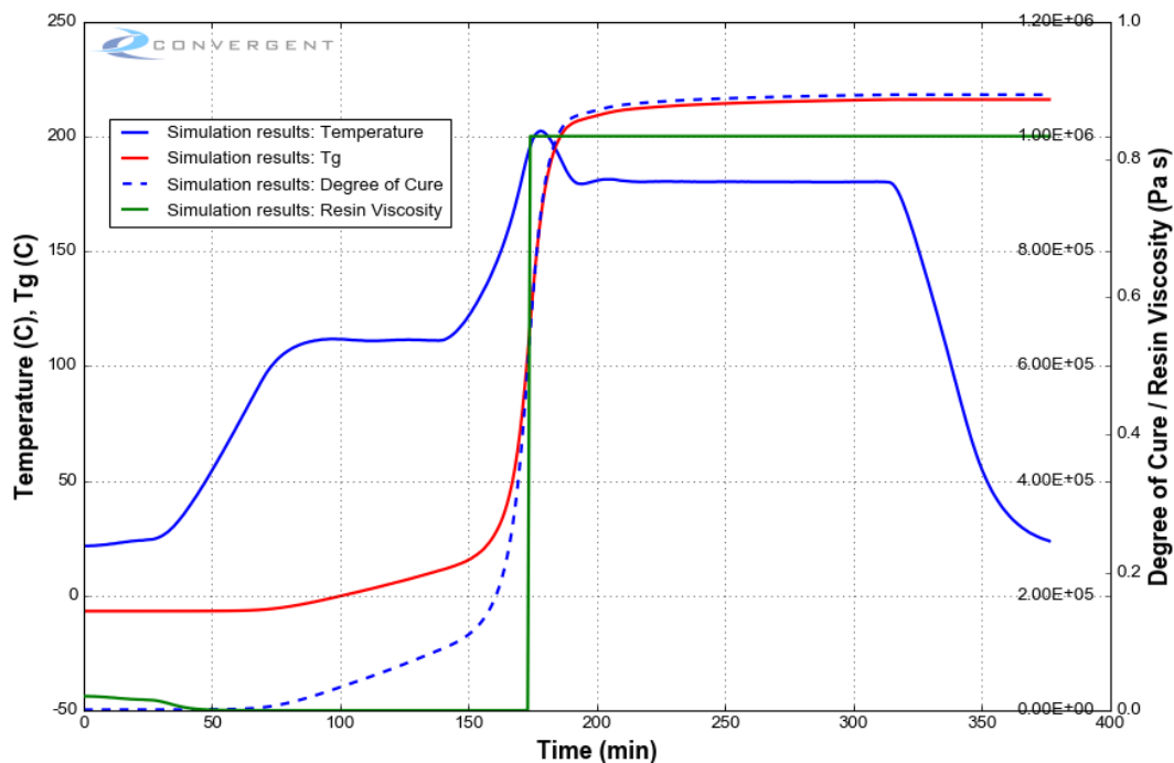
Figure 5.29: Sim_data: Simulation for Step 5 of cure cycle 1 based on thermocouple data from the centre of the step. The temperature profile from the thermocouple is the blue line. Degree of cure is on the external right axis and resin viscosity on the internal right axis.
