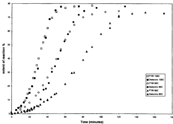
Figure 2.25: Degree of cure vs time as measured by DEA and FTIR spectroscopy. Reproduced from [67].
