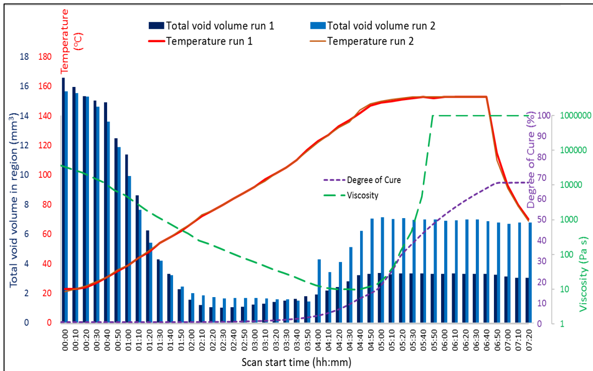
Figure 4.24: Defect evolution and resin behaviour, ply drop gap with \sim 150^{\circ}\text{C} hold. Resin behaviour calculated from the model of Kratz et al. [43]
