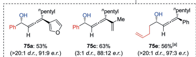
Scheme 14. Palladium-catalyzed enantioselective conjunctive cross-coupling reactions of enyne boronate complexes. [a] Using B(hac*) instead of Bpin. R_M = Migrating group.
