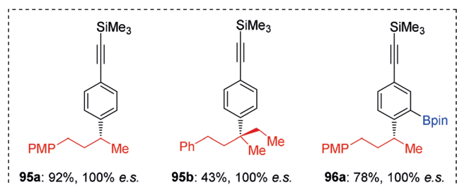
Scheme 18. Coupling boronic esters with phenylacetylenes via alkyne activation.
