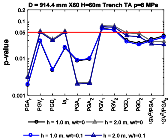
3 4 Fig. 20 Effect of burial depth, h , of the pipeline on p -values computed through regression analyses of 5 \varepsilon_{res} | IM relative to epicentral distances ( \ln(R) ) of the selected ground motions. Results for X60 D = 6 914.4 mm pipelines embedded in trench TA in soil subdeposits with depth H = 60 m.
