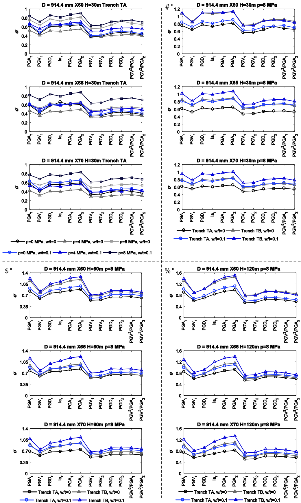
1 2 Fig. 12 Comparisons of standard deviations \sigma computed for D = 914.4\text{mm} pipelines through 3 regression analyses of the axial compression strain \epsilon of pipelines relative to tested seismic IMs . (a) 4 Effects of internal pressure p and pipeline wall imperfections ( w/t ) on \sigma values. (b) Effect of trench
