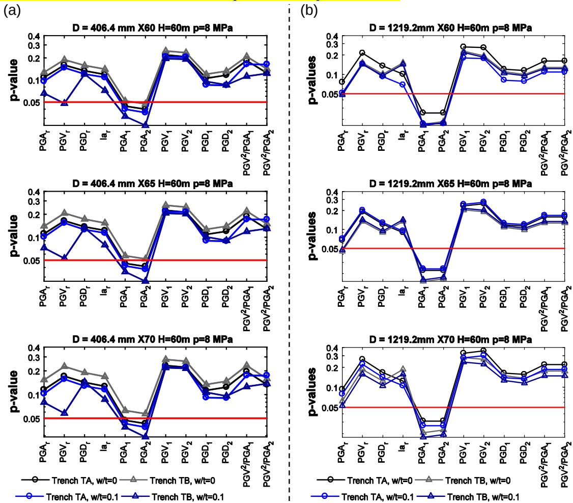
8 9 Fig. 18 Comparisons of p -values computed for (a) D = 406.4 mm and (b) D = 1219.2 mm pipelines 10 through regression analyses of \varepsilon_{res} | IM relative to magnitudes ( M ) of selected ground motions.
