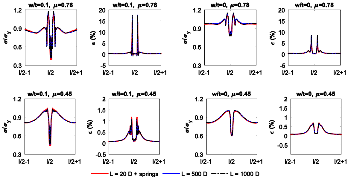
3 Fig. 7 Comparisons of axial stress (normalized over yield Mises stress) and axial strain along the ditch 4 axis of a D = 914.4 mm perfect (i.e. w/t=0 ) and imperfect (i.e. w/t=0.1 ) pipeline, embedded in trench 5 TA ( \mu = 0.45 ) or TB ( \mu = 0.78 ) at a burial depth h = 1.0 m, computed by the 3D SPI model with the 6 nonlinear springs at end-sides, (i.e. L = 20 D ) and extended 3D SPI models ( L = 500 D and L = 1000 7 D ), the latter simulating the ‘infinitely’ long soil-pipeline system.
