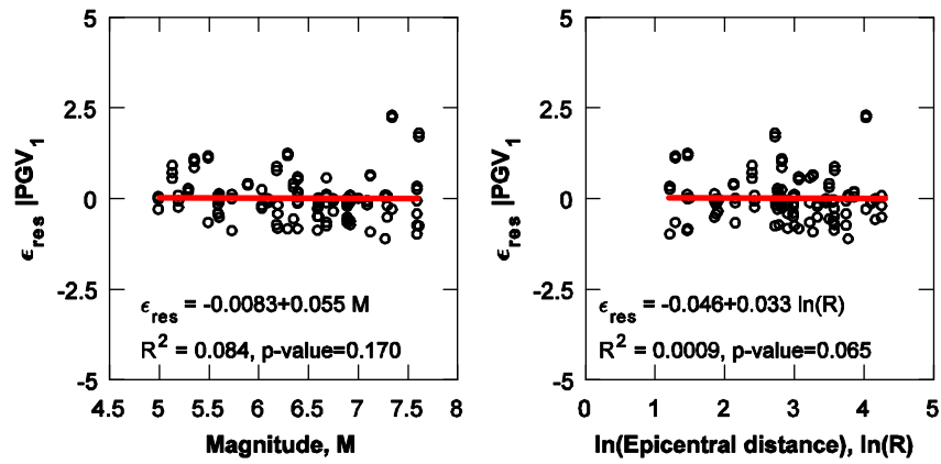
Fig. 15 Representative regression analyses of \epsilon_{res}|IM relative to magnitudes (M) and epicentral distances ( \ln(R) ) of selected ground motions, aiming at evaluating the sufficiency of PGV_1 . Results for X60 D = 914.4 mm ‘perfect’ pipelines, embedded in trench TA in soil deposits with depth H = 30 m and pressurized at p = 8 MPa.
