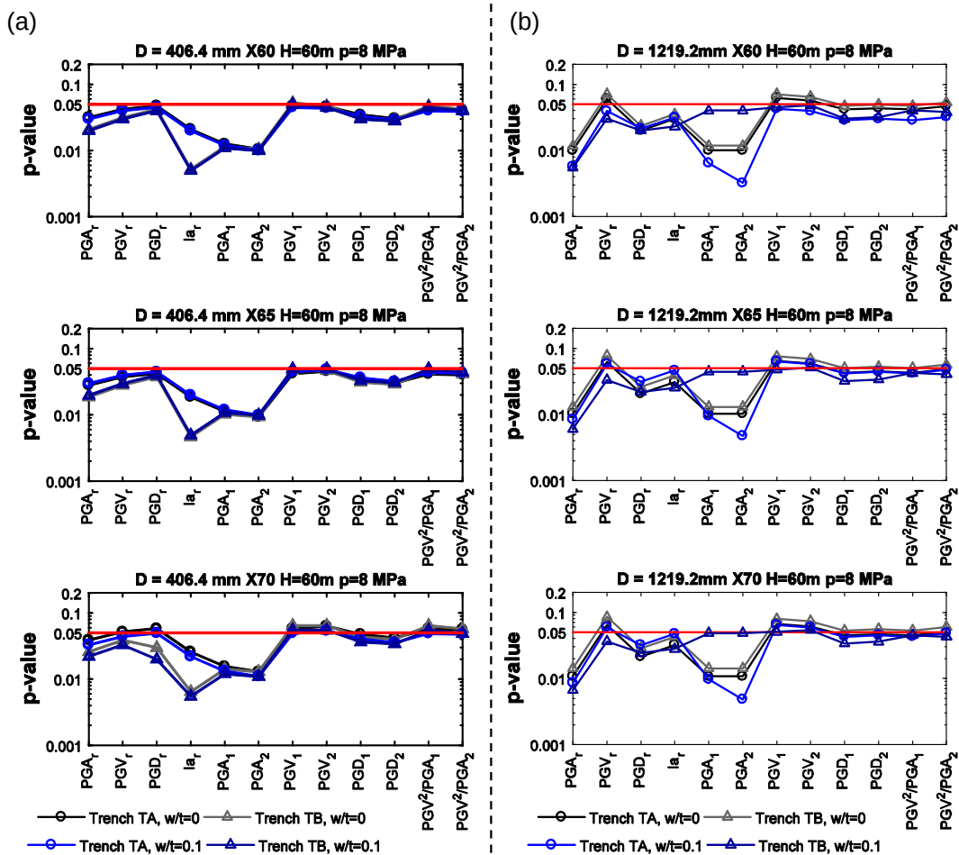
7 8 Fig. 21 Comparisons of p -values computed for (a) D = 406.4 mm and (b) D = 1219.2 mm pipelines 9 based on regression analyses of \varepsilon_{res} | IM relative to epicentral distances ( \ln(R) ) of the selected ground 10 motions.
