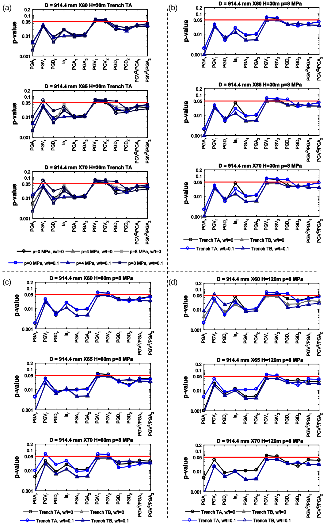
1 2 Fig. 19 Comparisons of p -values computed for all tested seismic IMs through regression analyses of 3 \varepsilon_{res} | IM relative to epicentral distances ( \ln(R) ) of the selected ground motions. (a) Effects of internal 4 pressure p and pipeline wall imperfections ( w/t ) on p -values. (b) Effects of trench properties and soil-
