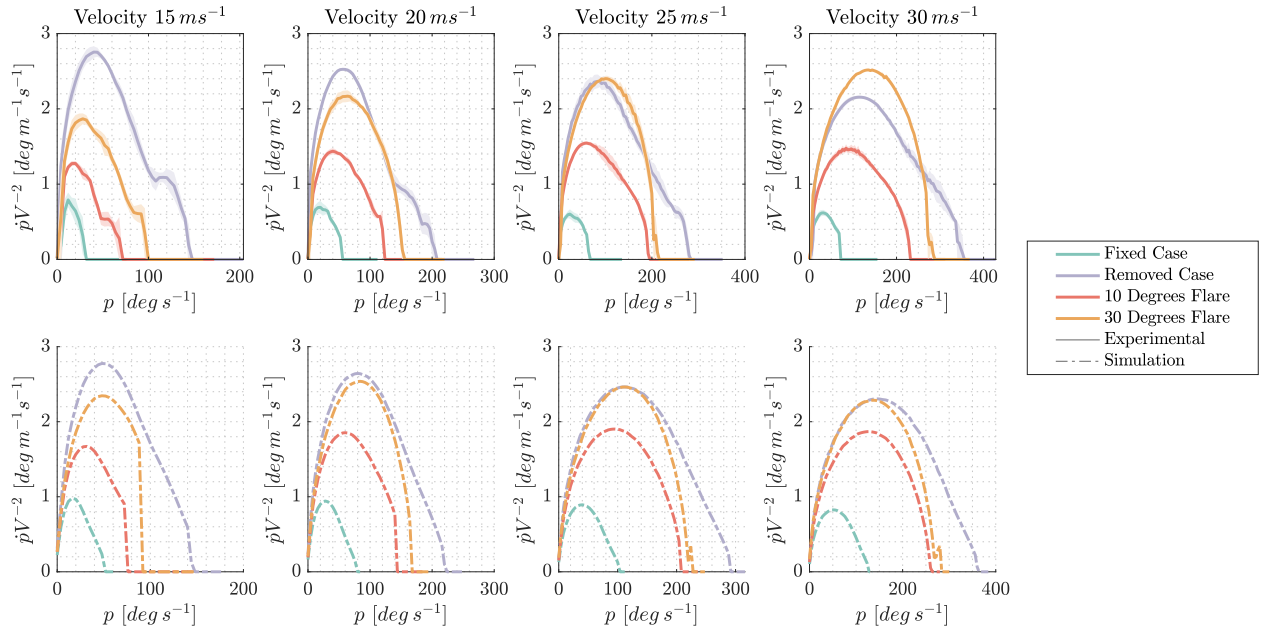
Fig. 21 A comparison of the experimental and simulated acceleration, velocity phase space for the each configuration
