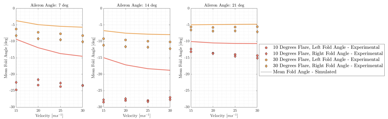
Fig. 11 The mean fold angle of each wingtip at each aileron angle and velocity for each model configuration
