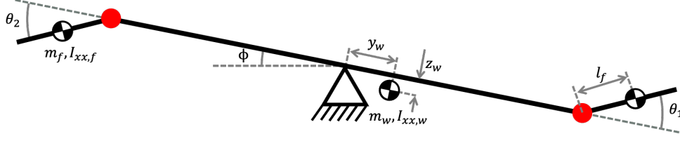
Fig. 5 Diagrammatic representation of the three degree of freedom mathematical model, as viewed from downstream of the model
