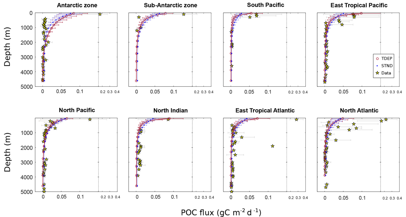
Figure 12. POC flux ( \text{gC m}^{-2} \text{d}^{-1} ) for the model (mean and standard deviation) and data. Data from Mouw et al. (2016a). STND is the standard model, and TDEP is the temperature-dependent model.
