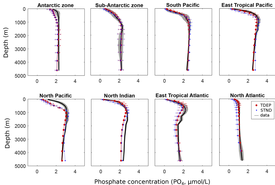
Figure 7. \text{PO}_4 ( \mu\text{molL}^{-1} ) per depth by region for the model and data (mean and standard deviation). Data from WOA 2009 (Levitus et al., 2010). STND is the standard model, an TDEP is the temperature-dependent model.
