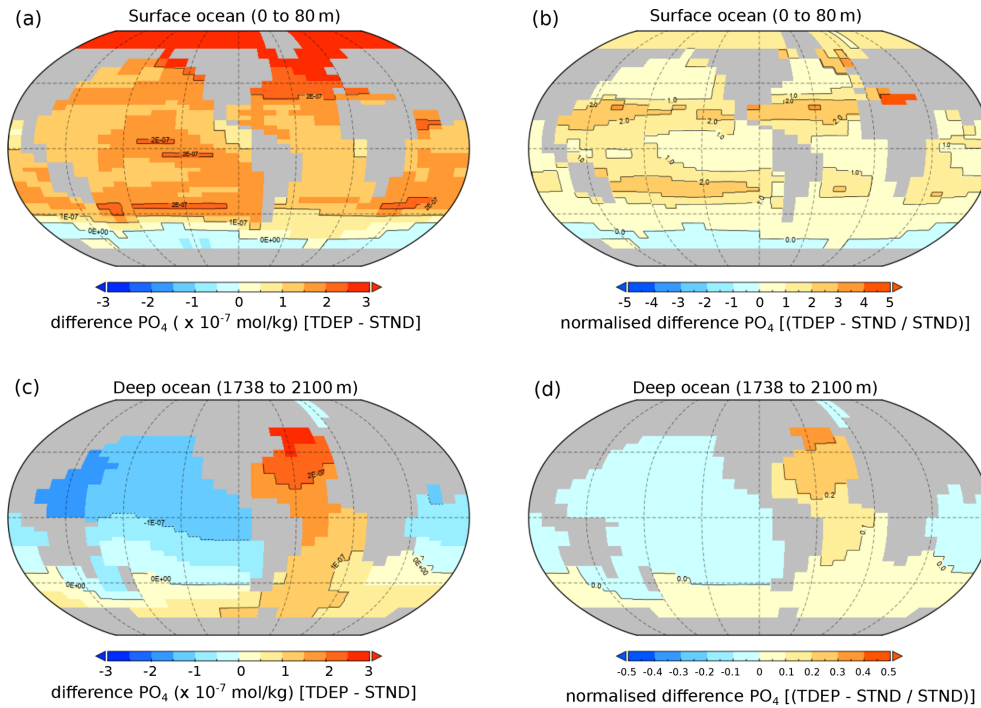
Figure 8. Difference in PO 4 concentration for best-fit TDEP compared to STND, (a, b) surface waters (0 to 80 m), and (c, d) deep waters (1738 to 2100 m). (a, c) Absolute difference (mol kg -1 ) and (b, d) normalised difference. All are the present day; note the scale difference in terms of the normalised difference between surface and deep water. STND is the standard model, and TDEP is the temperature-dependent model.
