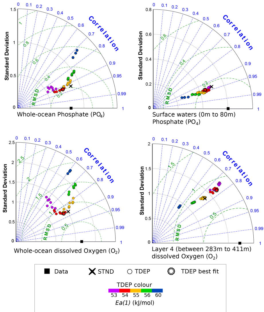
Figure 5. Taylor diagrams for the model fit to data for PO 4 and O 2 concentrations, showing the standard deviation (standard deviation is not normalised), correlation, and centred root means square difference (RMSD). Data from WOA 2009 (Levitus et al., 2010). The best-fit TDEP setting is double circled.
