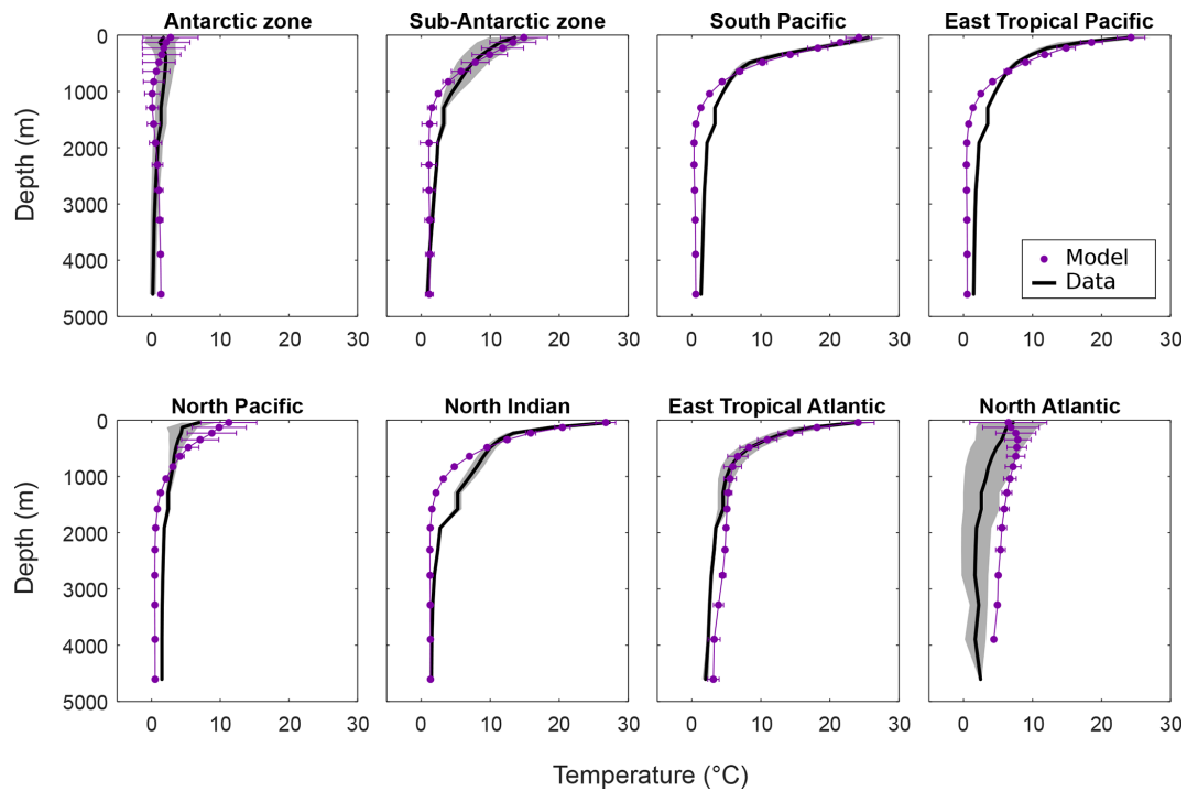
Figure 4. Temperature ( ^{\circ}\text{C} ) per depth by region for the model and data (mean and standard deviation). Data from WOA 2009 (Levitus et al., 2010).
