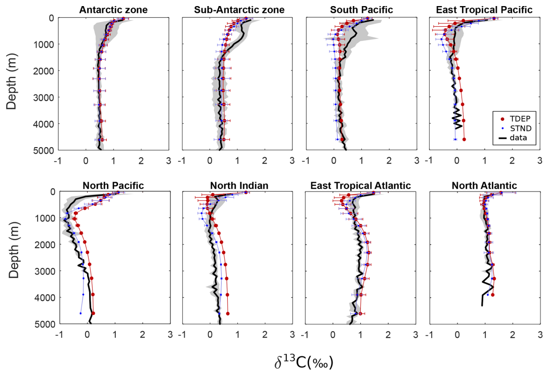
Figure 10. \delta^{13}\text{C} of DIC ( \text{‰ VPDB} ) per depth by region for the model and data (mean and standard deviation). Data from Schmittner et al. (2013). STND is the standard model, and TDEP is the temperature-dependent model.
