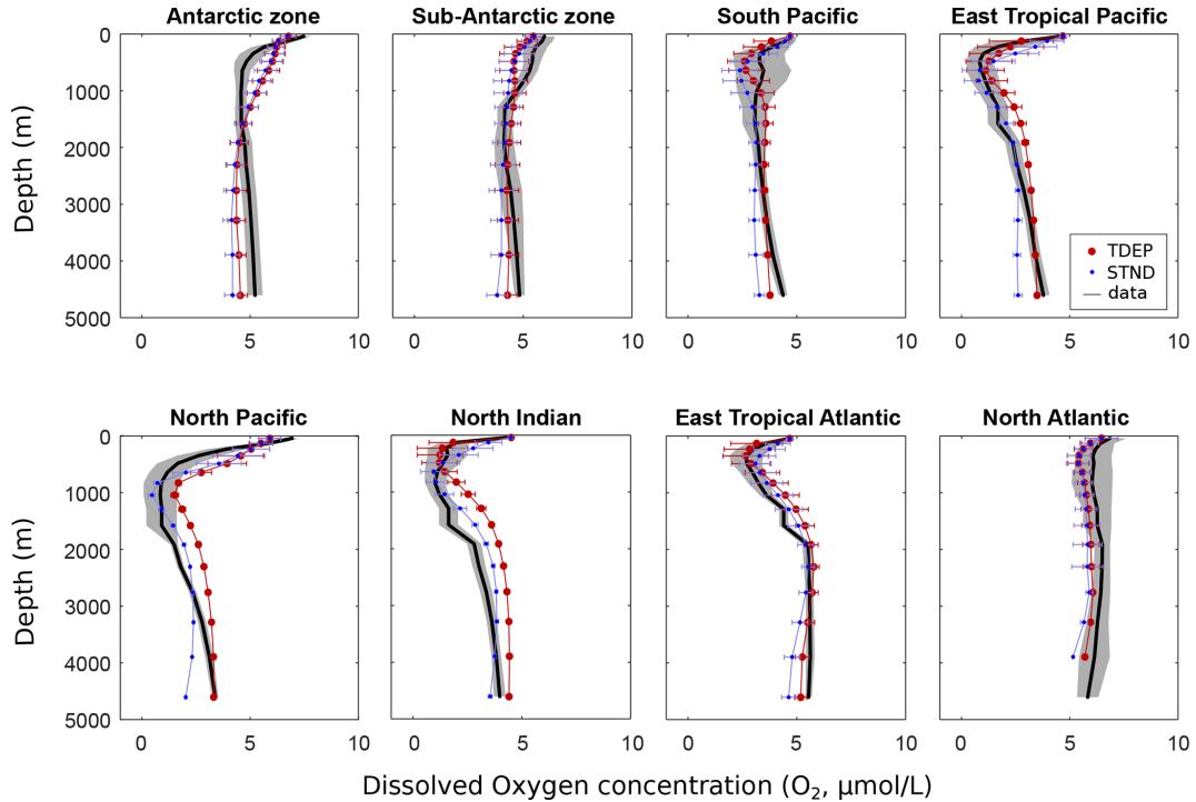
Figure 9. Dissolved O 2 (µmol L -1 ) per depth by region for the model and data (mean and standard deviation). Data from WOA 2009 (Levitus et al., 2010). STND is the standard model, and TDEP is the temperature-dependent model.
