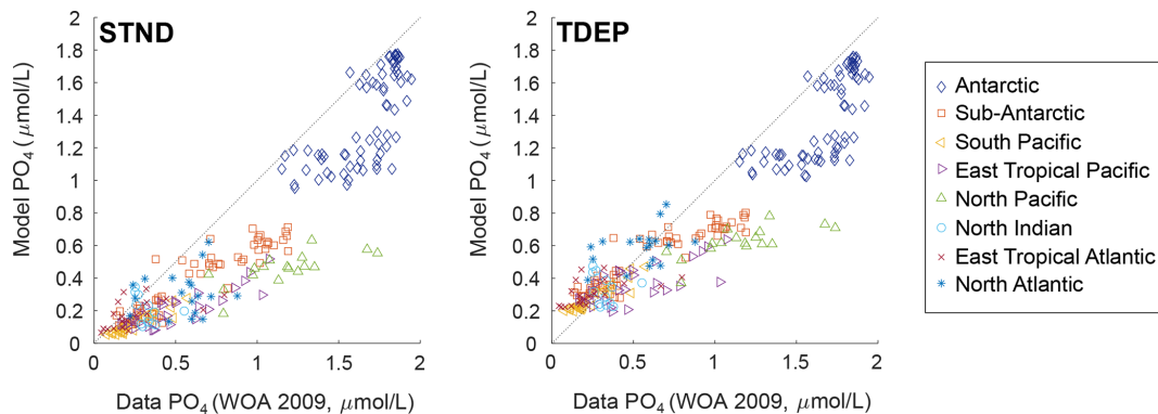
Figure 6. Cross-plot for surface (0 to 80 m) PO 4 concentrations (µmolL -1 ) for the data and model labelled by ocean region. Data from WOA 2009 (Levitus et al., 2010).
