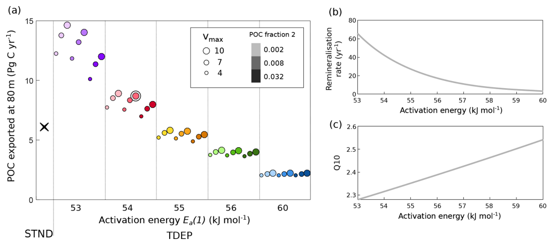
Figure 11. Global POC flux ( \text{Pg C yr}^{-1} ) at 80 m (a) and the effect of activation energy on (b) remineralisation rate and (c) Q_{10} (for a 0 to 10^\circ\text{C} change). In (a) the STND model is shown as a black cross, and the TDEP model is indicated by circles. The best-fit TDEP setting is double circled. STND is the standard model, and TDEP is the temperature-dependent model. Colours in (a) reflect those used in Fig. 5.
