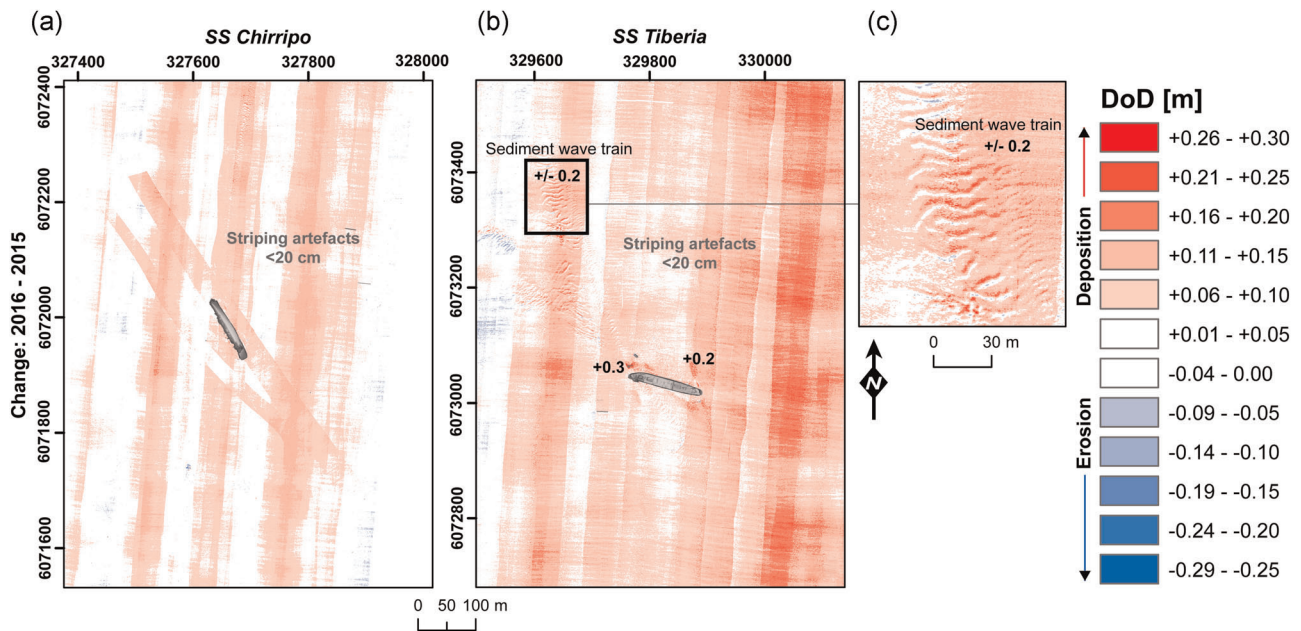
FIGURE 9 Annual digital elevation models of difference (2016–2015) with minor geomorphic changes for (a) SS Chirripo , (b) SS Tiberia , and (c) inset map showing a sediment wave train in SS Tiberia 's far field. Pixels within the detection threshold ( \pm 30 cm) were retained to avoid information loss [Color figure can be viewed at wileyonlinelibrary.com ]
