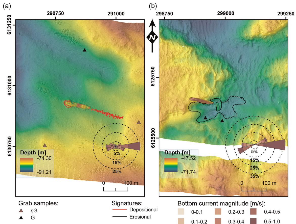
FIGURE 5 Gravel-dominated sites presented as digital elevation models with a multidirectional hillshade occlusion: (a) SS Lugano , (b) SS Santa Maria . Rose charts represent the modeled near-seabed current data. Grab samples: G, gravel; sG, sandy gravel [Color figure can be viewed at wileyonlinelibrary.com ]
