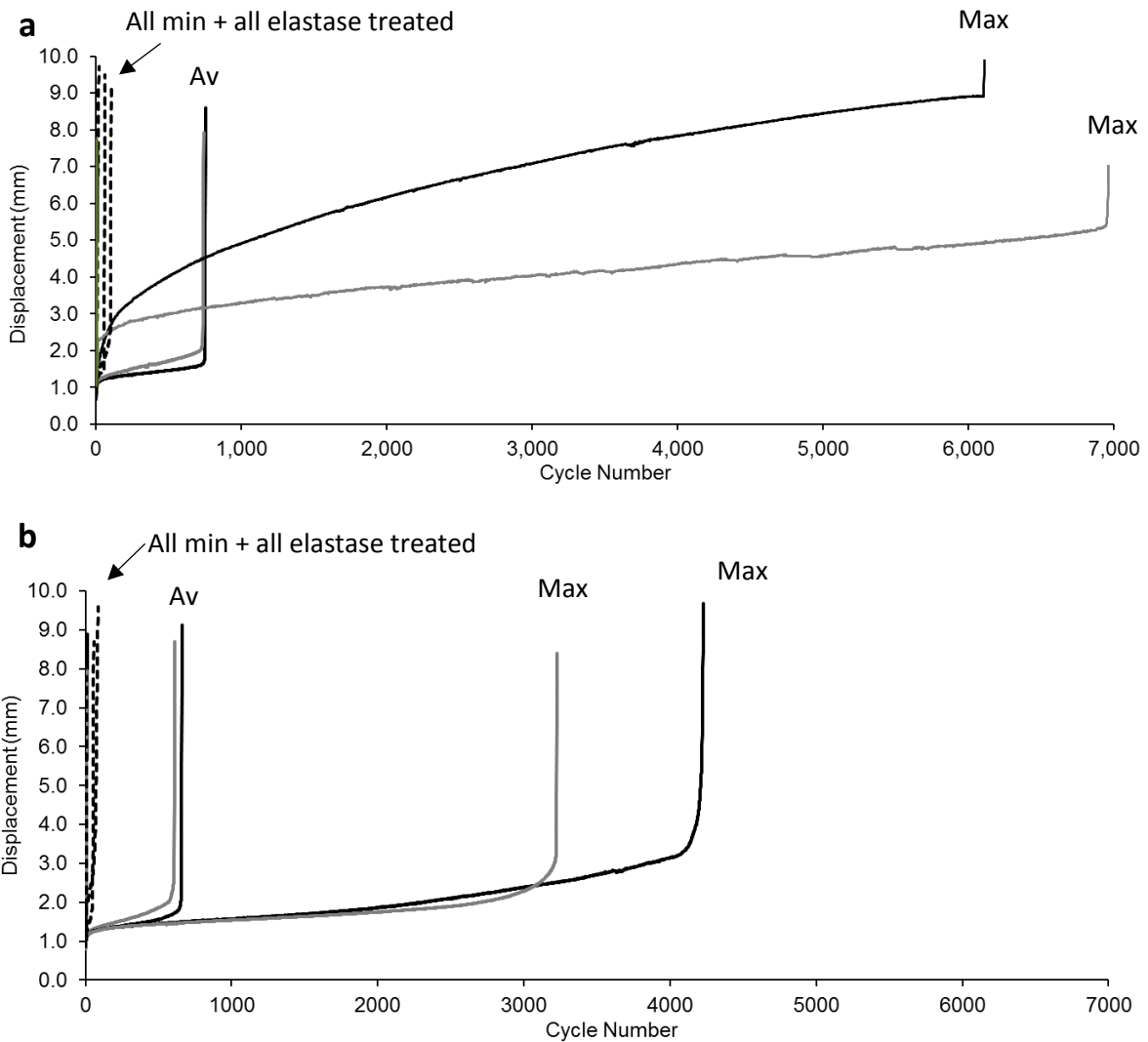
Figure 3 - Creep curves of young SDFT IFM (a) and old SDFT IFM (b), highlighting the variability between samples by plotting the maximum (Max) and minimum (Min) curves in each group, alongside the average (Av). Fresh samples are shown in black, control samples in grey, elastase treated with a dotted line. Labelling is not used for elastase treated samples as it evident all elastase treated samples failed at less than 100 cycles.
