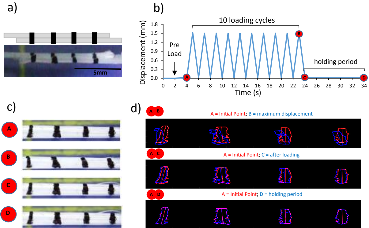
Figure 1 - Schematic showing IFM recovery testing protocol.
