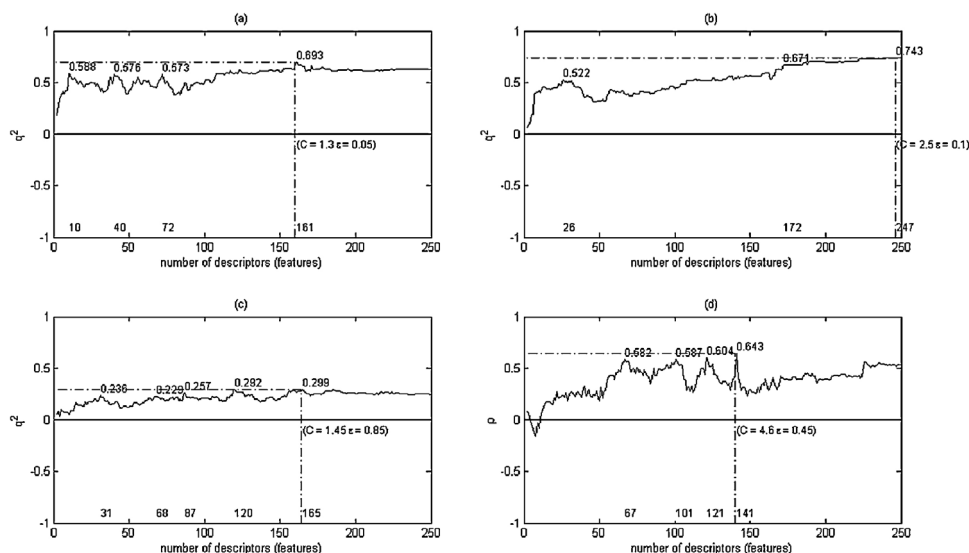
Fig. 6. The performance of 4-rule fuzzy model based on the number of descriptors. (a) Task 1: Graph reaches highest peak at 161 with the SVR parameters ( C=1.3 and \epsilon=0.05 ). (b) Task 2: Graph reaches highest peak at 247 with the SVR parameters ( C=2.5 and \epsilon=0.1 ). (c) Task 3: Graph reaches highest peak at 165 with the SVR parameters ( C=1.45 and \epsilon=0.85 ). (d) Task 4: Graph reaches highest peak at 141 with the SVR parameters ( C=4.6 and \epsilon=0.45 ).
