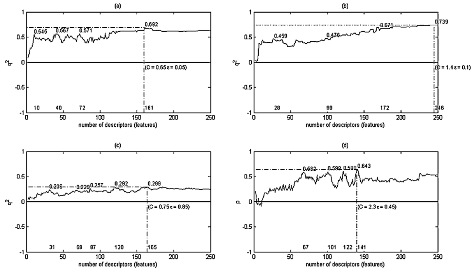
Fig. 4. The performance of 2-rule fuzzy model based on the number of descriptors. (a) Task 1: Graph reaches highest peak at 161 with the SVR parameters ( C = 0.65 and \epsilon = 0.05 ). (b) Task 2: Graph reaches highest peak at 246 with the SVR parameters ( C = 1.4 and \epsilon = 0.1 ). (c) Task 3: Graph reaches highest peak at 165 with the SVR parameters ( C = 0.75 and \epsilon = 0.85 ). (d) Task 4: Graph reaches highest peak at 141 with the SVR parameters ( C = 2.3 and \epsilon = 0.45 ).
