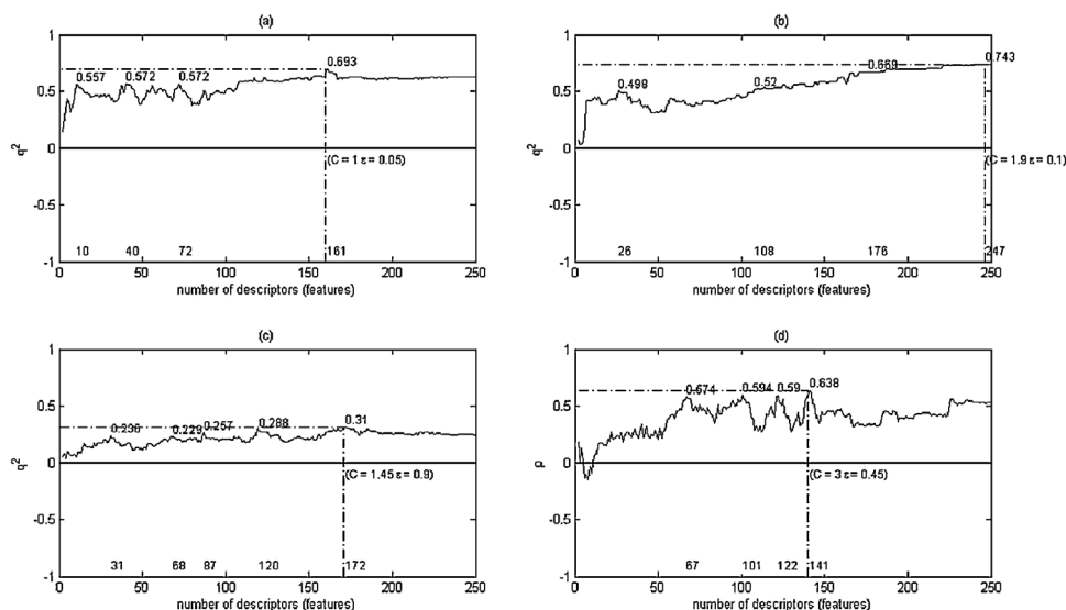
Fig. 5. The performance of 3-rule fuzzy model based on the number of descriptors. (a) Task 1: Graph reaches highest peak at 161 with the SVR parameters ( C=1.0 and \epsilon=0.05 ). (b) Task 2: Graph reaches highest peak at 247 with the SVR parameters ( C=1.9 and \epsilon=0.1 ). (c) Task 3: Graph reaches highest peak at 172 with the SVR parameters ( C=1.45 and \epsilon=0.9 ). (d) Task 4: Graph reaches highest peak at 141 with the SVR parameters ( C=3.0 and \epsilon=0.45 ).
