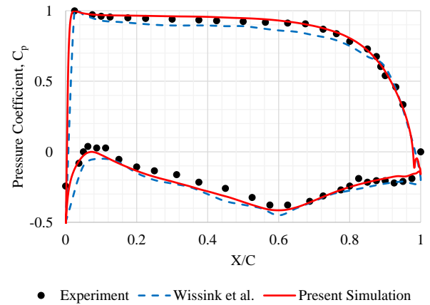
FIGURE 2: TIME-AVERAGED PRESSURE COEFFICIENT DISTRIBUTIONS
