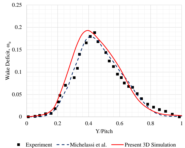
FIGURE 3: WAKE LOSS PROFILES
