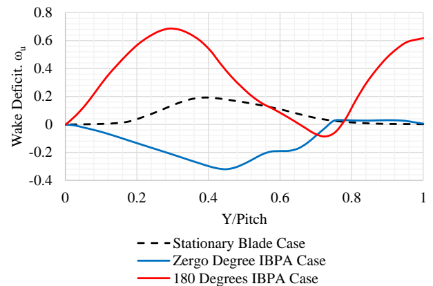
FIGURE 9: WAKE PROFILES
