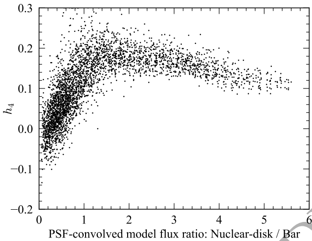
Figure 19. MUSE stellar-kinematic h_4 values for 12 \times 12'' central region of NGC 4643, plotted against the local ratio of our nuclear-disc model to the rest of the bar model. The h_4 values peak where the ratio is \sim 1 , suggesting that the high kurtosis is the result of nearly equal contributions from nuclear-disc and bar LOSVDs with significantly different dispersions.
