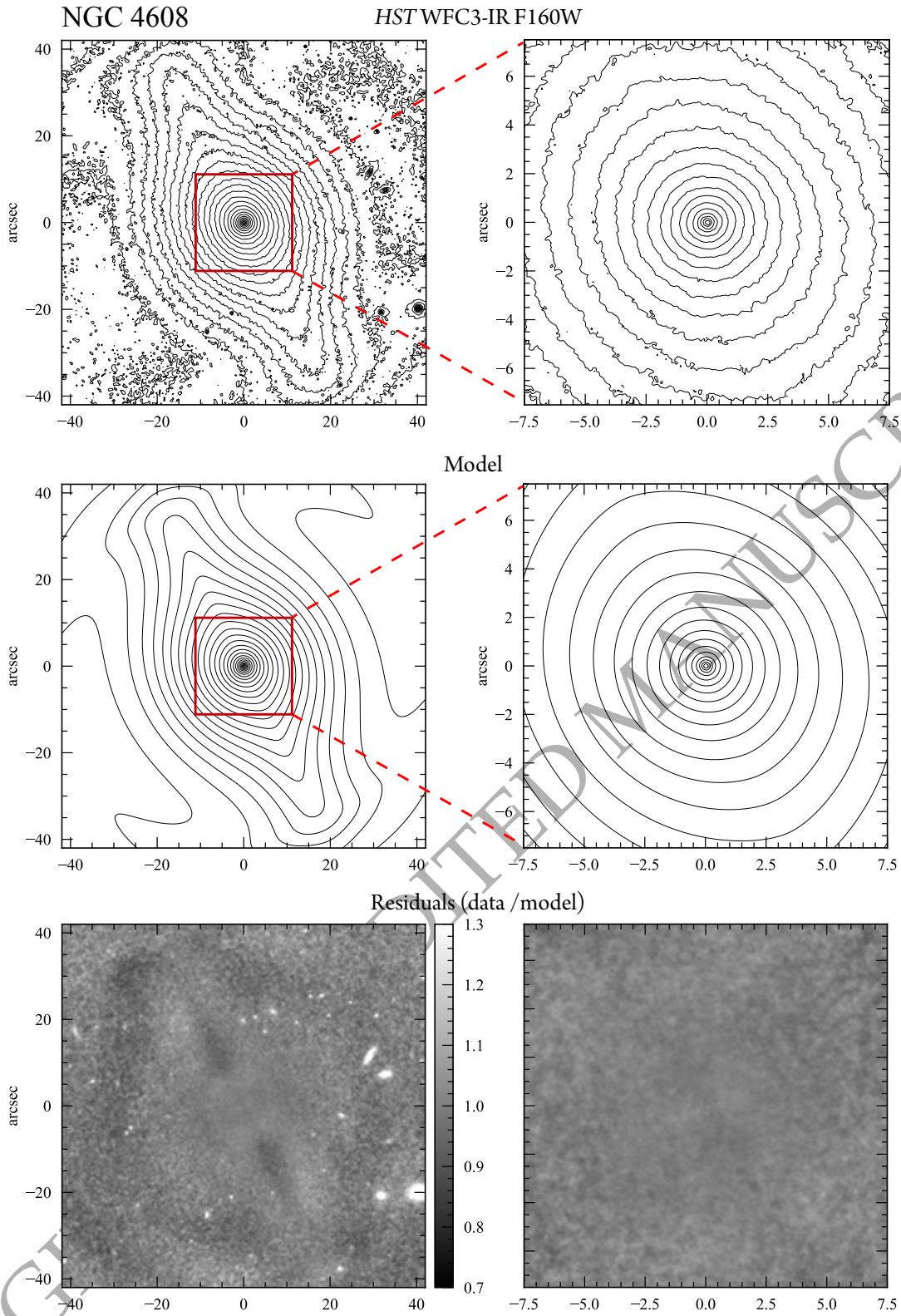
Figure 7. Best-fitting model for NGC 4608, compared with HST WFC3-IR F160W image. Upper and middle panels show logarithmically spaced isophotes from F160W image (top) and best-fitting model (middle); bottom panels show residuals (data values divided by model values). The large-scale images (left) were smoothed using a 9 \times 9 -pixel-wide median filter.
