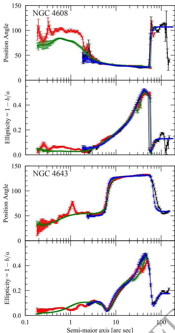
Figure 4. Ellipse fits to Spitzer IRAC1 images (black) and HST F160W images (red) of both galaxies (top: NGC 4608; bottom: NGC 4643), along with ellipse fits to the best-fitting model images (blue = model fit to IRAC1 image, green = model fit to F160W image).
