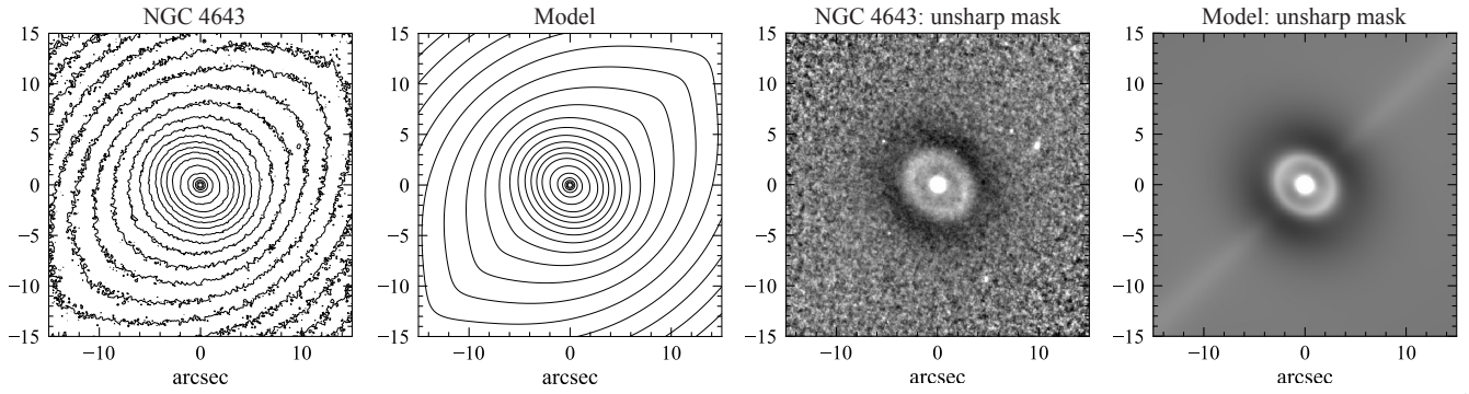
Figure 11. Comparison of the nuclear-disc region of NGC 4643 with our best-fitting model. Left two panels: Logarithmically spaced isophotes for the E160W image of NGC 4643 (left) and our model (right). Right two panels: Unsharp masks of the same (made using a Gaussian with \sigma = 15 pixels). Note the clearly ringlike feature in the unsharp masks, produced (in the model, at least) by the abrupt change in slope of the nuclear disc rather than by a separate nuclear ring.
