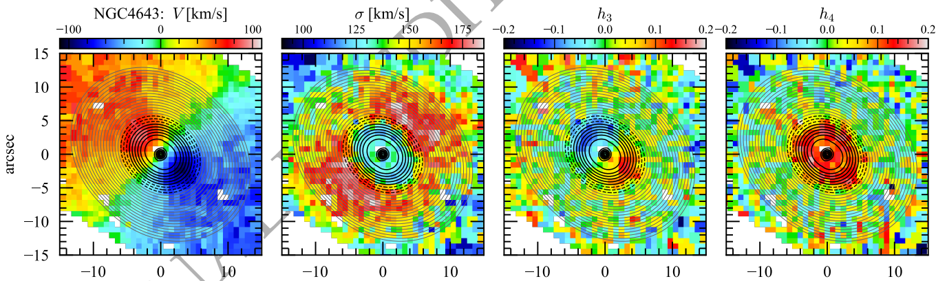
Figure 16. A close-up of the lower panels (ATLAS 3D stellar kinematics) of Figure 15, but with contours now showing the ratio of the nuclear-disc component to the rest of our best-fitting model of NGC 4643 (e.g., Figure 10). Solid black contours indicate where the nuclear disc is brighter, dashed black contours where its brightness is 50–100% of the rest of the model, and thin grey contours where it is fainter. Note that the region dominated by the nuclear-disc component matches almost perfectly with the fast rotation, lower velocity dispersion, strong V - h_3 anticorrelation, and enhanced h_4 .
