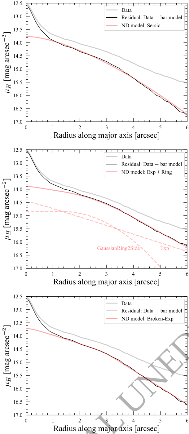
Figure A1. Profiles from major-axis cuts through the F160W image of NGC 4643 (thick grey lines) and through residual images (black lines), formed by subtracting the bar components of the best fitting model. All models are identical except for how the nuclear-disc region is represented. In all three cases, the residuals in the nuclear-disc region show similar broken-exponential profiles with a break at r \sim 3'' , indicating that this is a robust feature of the galaxy. Upper panel: Best-fitting model uses Sérsic component for nuclear disc. Middle panel: Best-fitting model uses Exponential + GaussianRing2Side components for nuclear disc. Lower panel: Best-fitting model uses BrokenExponential component for nuclear disc (this is the model discussed in the main text of the paper).
