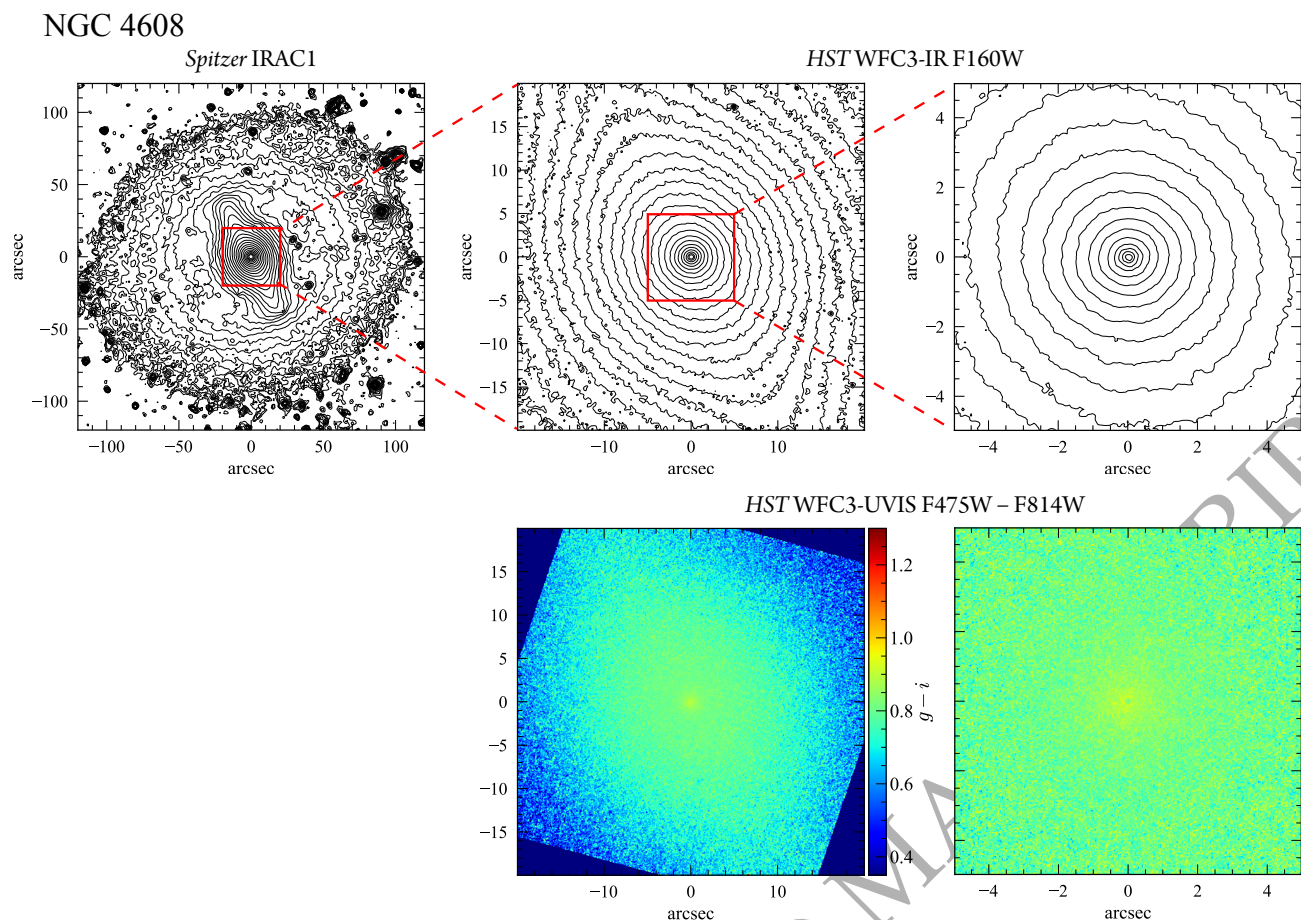
Figure 2. Imaging overview of NGC 4608. Top row: from left to right, logarithmically spaced Spitzer IRAC1 isophotes (left, median-smoothed with width = 5 pixels, contour spacing of 0.1 des) and two close-ups showing HST WFC3-IR F160W isophotes (middle, median-smoothed with same width; right, unsmoothed). Bottom row: HST WFC3-UVIS colour maps (F475W – F814W, converted to g-i ) on the same spatial scales and smoothing as the corresponding F160W isophote plots. (Unless otherwise explicitly noted, all figures in this paper have standard astronomical orientation: N = up, E = left)
