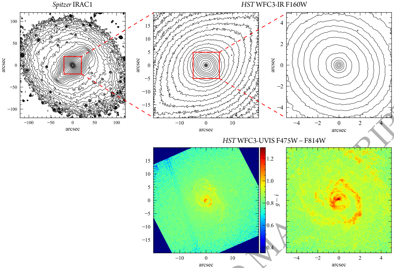
Figure 3. Same as Figure 2, but now showing NGC 4643.
