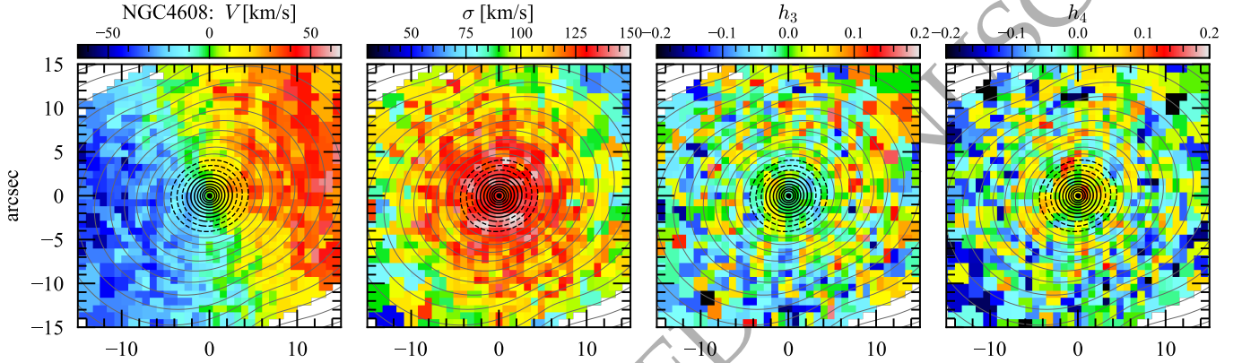
Figure 14. A close-up of Figure 13, but with contours now showing the ratio of the classical-bulge (Sérsic) component to the rest of our best-fitting model of NGC 4608 (e.g., Figure 7). Solid black contours indicate where the classical-bulge component is brighter, dashed black contours where its brightness is 50–100% of the rest of the model, and thin grey contours where it is fainter. The region dominated by the bulge component has almost no rotation, centrally increasing velocity dispersion, and little or no signature in h_3 or h_4 ; this is suggestive of a classical bulge.
