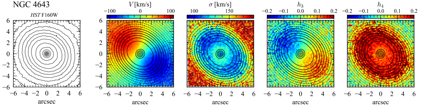
Figure 18. MUSE stellar kinematics for the nuclear-disc region of NGC 4643. Leftmost panel: Isophotes from F160W image of NGC 4643. Middle and right panels: Stellar kinematics for NGC 4643, from single-spaxel analysis of VLT-MUSE data. Contours in these panels are as in Figure 16: solid contour lines indicate where the nuclear-disc component of our best-fitting model is brighter, dashed black contours where its brightness is 50–100% of the rest of the model, and thin grey contours where it is fainter (note that the inner four solid contour lines indicate decreasing levels of relative brightness toward the center, due to the increasing importance of the compact classical-bulge/NSC component). The nuclear-disc ratio image has been convolved to match the FWHM \approx 0.75'' seeing of the MUSE kinematics.
