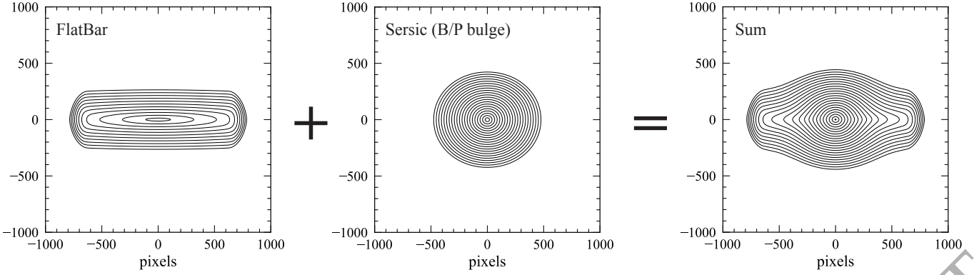
Figure B1. The IMFIT components of our bar model. Left: the new “FlatBar” component, representing a face-on or low-inclination view of the vertically thin part of the bar. Middle: a mildly elliptical Sérsic component ( n = 1 ), representing the face-on/low-inclination view of the B/P bulge. Right: the sum of the two. (All isophotes are logarithmically spaced.)
