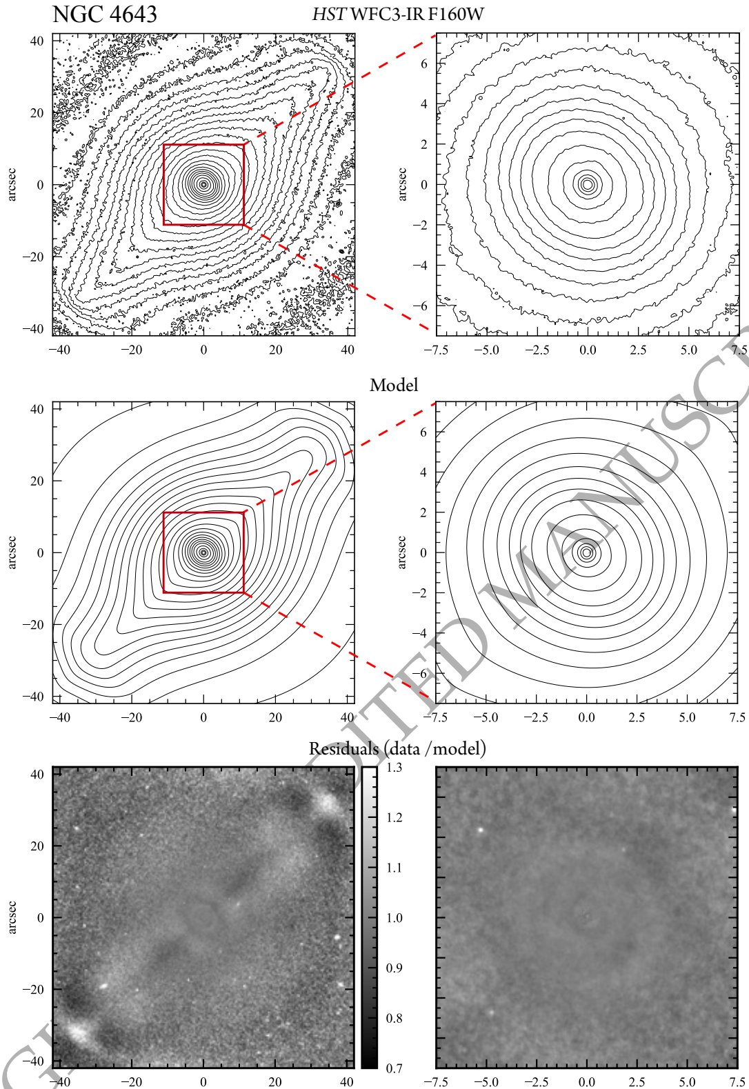
Figure 10. Best-fitting model for NGC 4643, compared with HST WFC3-IR F160W image. Upper and middle panels show logarithmically spaced isophotes from F160W image (top) and best-fitting model (middle); bottom panels show residuals (data values divided by model values). The large-scale images (left) were smoothed using a 9 \times 9 -pixel-wide median filter.
