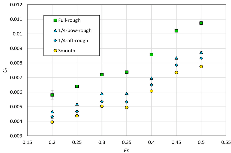
Fig. 6. values of Wigley model in smooth and 1/4-rough condition.
