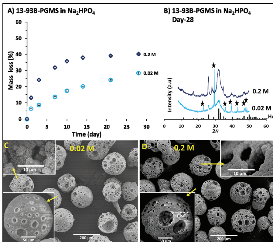
Fig. 9 (A) Highlights mass loss for PGMS of 13-93B in (0.02 M and 0.2 M) Na_2HPO_4 versus immersion time (days), (B) shows the X-ray diffraction patterns at day 28 and SEM images for PGMS of 13-93B post immersion of microspheres in (C) 0.02 M Na_2HPO_4 and (D) 0.2 M Na_2HPO_4 solution at 37 °C at day-28. Inset images show microspheres at higher magnification. XRD spectra for HA shown at the bottom of B for comparison. ★ highlights peaks for calcium carbonate ( CaCO_3 ).
