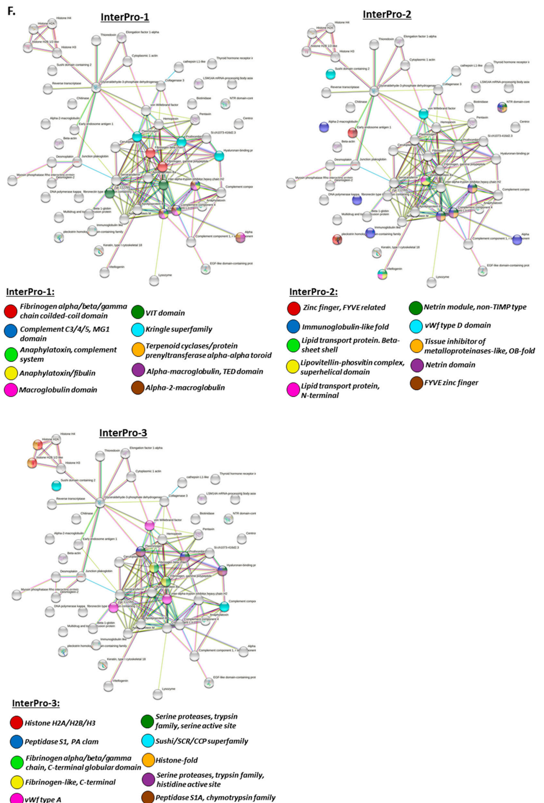
Figure 5. (A) Protein interaction networks for total protein cargo in halibut EVs, showing local network clusters. The coloured nodes indicate the different networks, respectively. (B) Reactome protein interaction networks for total proteins in halibut EV cargo, showing reactome pathways. Specific reactome pathways are indicated by the coloured nodes, respectively. (C) UniProt protein interaction networks for total proteins in halibut EV cargo, showing UniProt keywords. UniProt keywords are indicated by the coloured nodes, respectively. (D) PFAM protein interaction networks for total proteins in halibut EV cargo. The specific PFAM protein domains are indicated by
