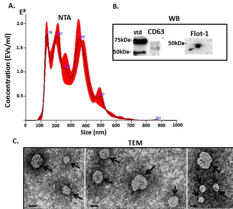
Figure 1. Halibut serum-extracellular vesicles (EV)s were characterised by: (A) Nanoparticle tracking analysis (NTA), showing size distribution profiles of EVs in the size range of 50–600 nm, with the modal size of vesicles at 138 nm; (B) Western blotting (WB) analysis shows that the EVs are positive for CD63 and Flotillin-1; (C) Transmission electron microscopy (TEM) showing EV morphology—see arrows pointing at EVs (scale bar is indicated at 20 nm).
