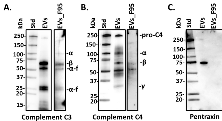
Figure 3. Complement component C3, C4 and pentraxin-like protein in halibut EVs and F95 enriched EV fractions. Western blotting showing (A) complement component C3 detection in total protein cargo of halibut serum-EVs (“EVs”) and in F95-enriched protein fractions from serum-EVs (“EVs_F95”), C3 \alpha - and \beta -chains, as well as \alpha -fragment ( \alpha -f) are indicated; (B) complement component C4 detection in total protein cargo of serum-EVs (“EVs”) and lower detection observed in F95-enriched EV protein fractions (“EVs_F95”), C4 \alpha -, \beta - and \gamma -chains are indicated; (C) pentraxin-like protein detection in total EV protein cargo (“EVs”), which was not detected in the F95-enriched EV protein fractions (“EVs_F95”).
