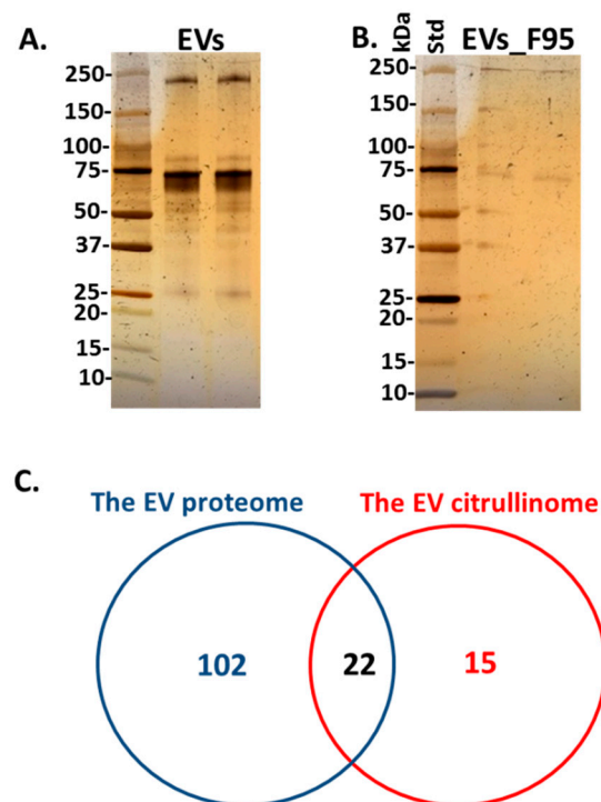
Figure 2. The proteome and citrullinome of halibut serum-EVs. Silver-stained gels for: (A) total protein cargo in EVs and (B) F95 enriched (deiminated/citrullinated) proteins from EVs. The protein standard (std) is indicated in kilodaltons (kDa). (C) Venn diagram shows the number of candidate protein hits identified as cargo in total serum EVs (“The serum EV proteome”) as well as deiminated protein hits in EV cargo (the serum “EV citrullinome”).
