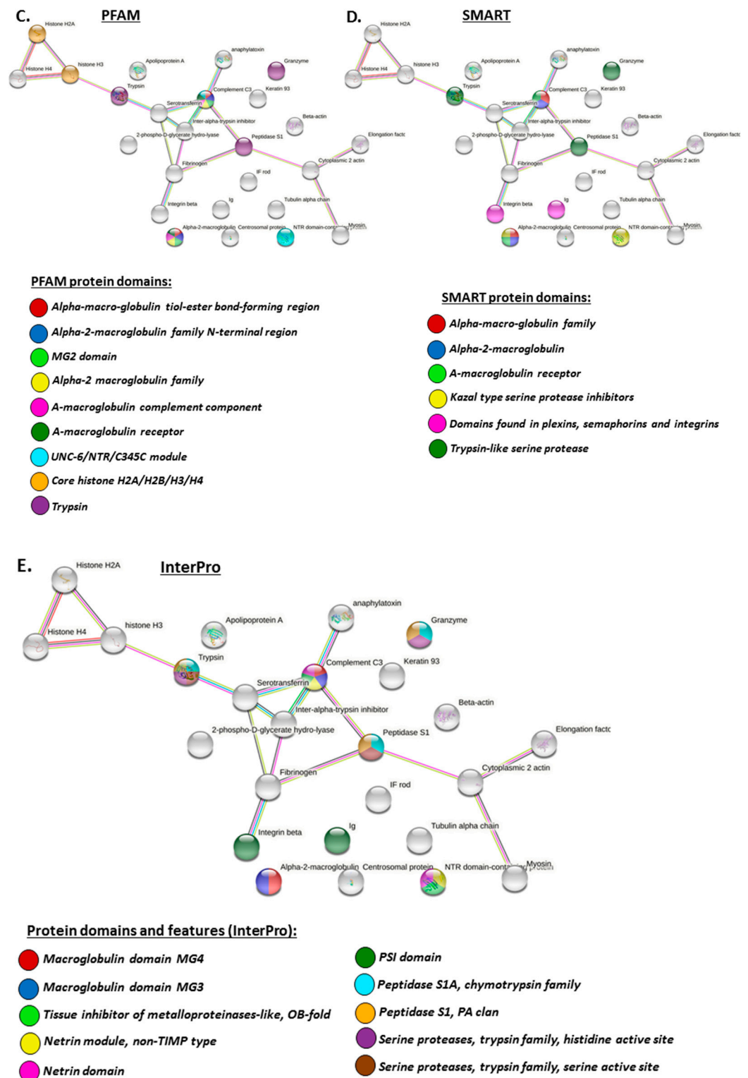
Figure 4. (A) Protein interaction networks for deiminated proteins in halibut EVs. Local network clusters and UniProt keywords are indicated by the colour coded nodes. See colour key for nodes and interaction networks in the figure. (B) Reactome protein interaction networks for deiminated proteins in halibut EVs. Reactome pathways are indicated by the coloured nodes, as shown in the figure. (C,D) PFAM and SMART protein interaction networks for deiminated proteins in halibut EVs. PFAM and SMART protein domains are indicated by the coloured nodes, see colour code in the figure. (E) InterPro protein interaction networks for deiminated proteins in halibut EVs. InterPro protein domains and features are indicated by the coloured nodes; see colour code in the figure.
