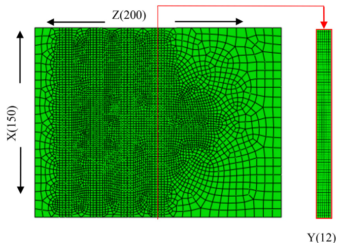
Fig. 7. Design of 3D finite element model of the TG6 benchmark specimen for contour residual stress measurement simulations. Dimensions are in mm.
