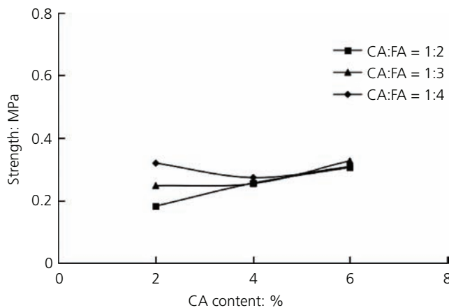
Figure 6. Influence of FA/CA ratio on UCS
