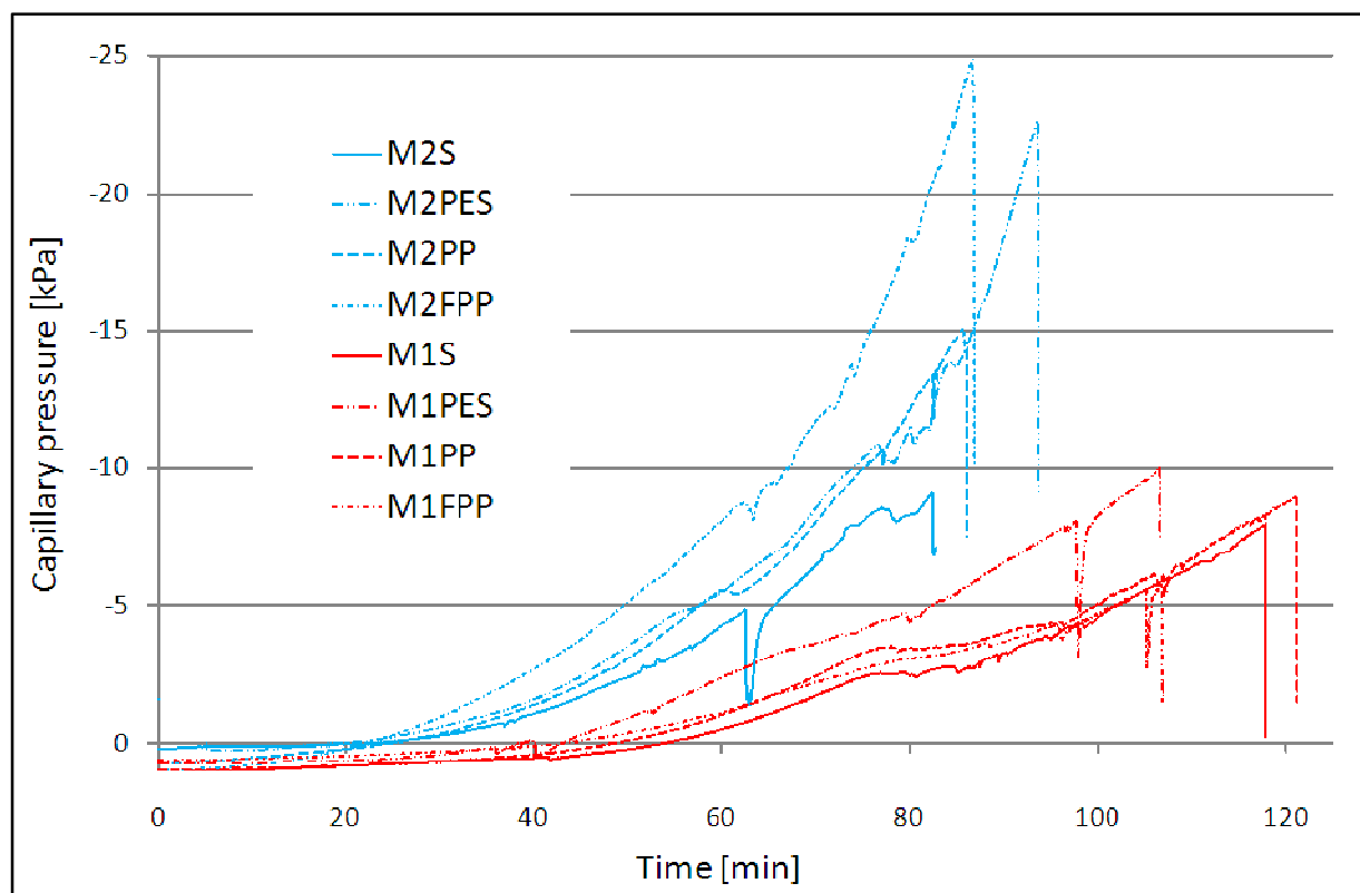
Figure 5.5: Capillary pressure of the standard Mixes 1 and 2 with and without fibres at Climate 1
