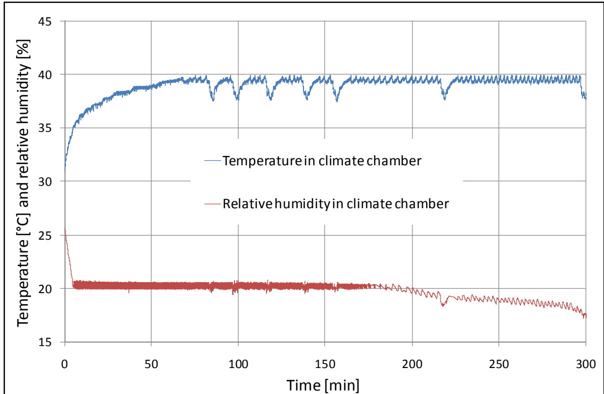
Figure A8: Climate chamber temperature and relative humidity for a mix with minimum bleeding under high wind speed
