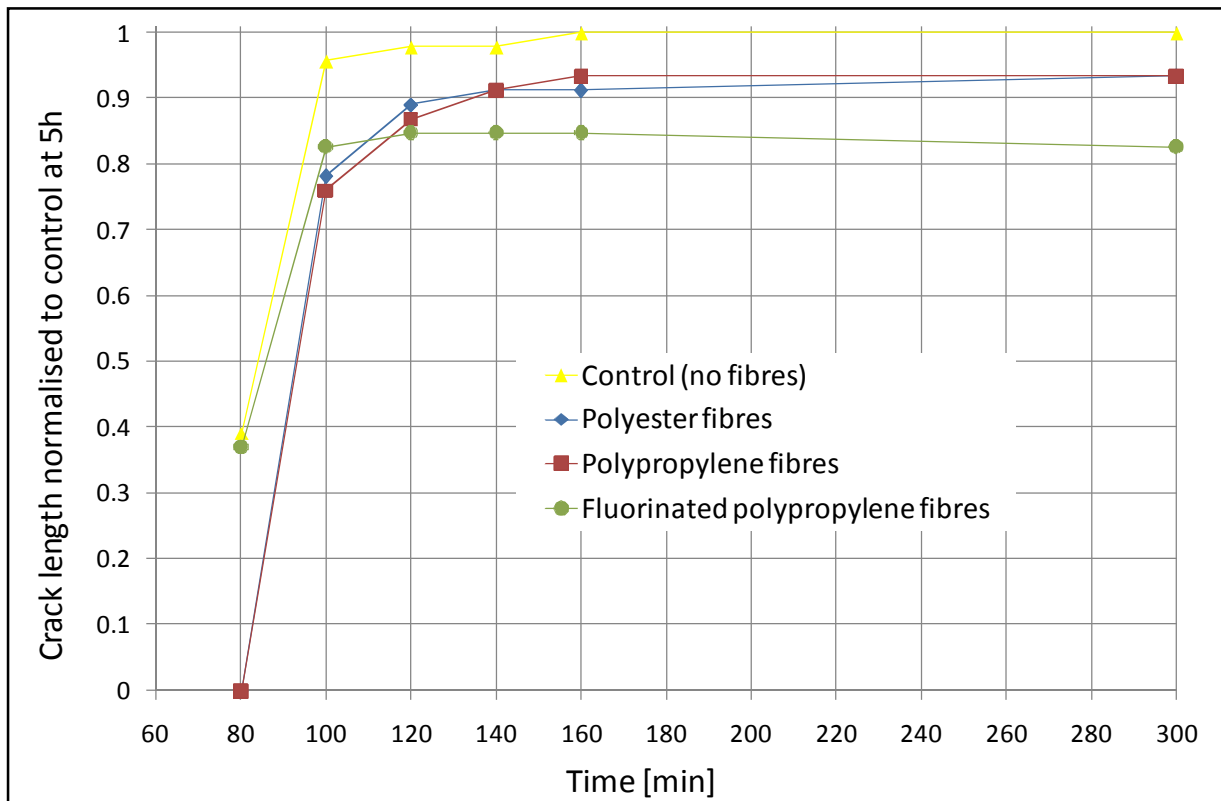
Figure 5.8: Normalised crack length for the standard Mix 2 with and without fibres at Climate 1
