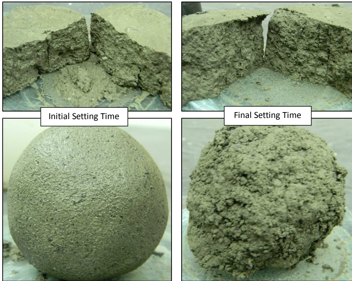
Figure 2.5: Pictures of a concrete paste at the initial and final setting times
