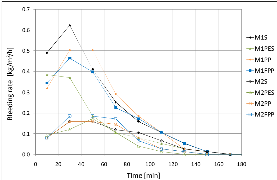
Figure 4.13: Bleeding rate of the standard Mixes 1 and 2 with and without fibres
