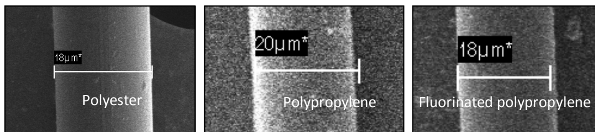
Figure 3.14: Electron microscope pictures of uncut fibre types
