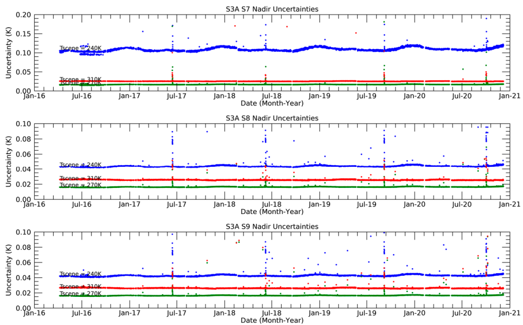
Figure 14. Time series for the period from March 2016 to December 2020 of SLSTR-A Thermal Infrared Radiometric Uncertainties (systematic effects) for scene temperatures of 240 K (blue), 270 K (green) and 310 K (red).
