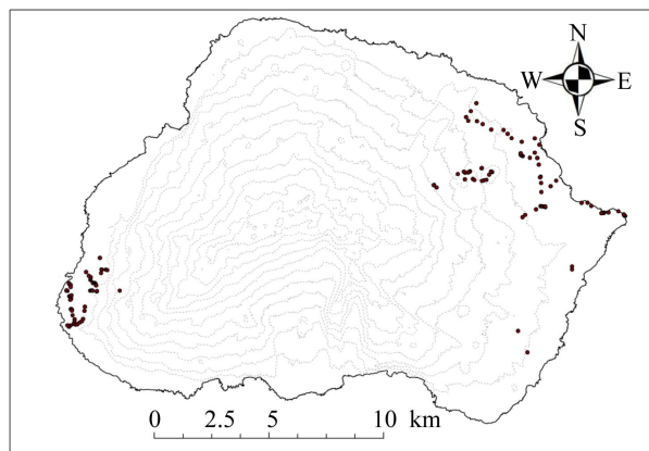
Figure 1. Map of Marion island with 100 m contour lines and showing localities where soils were sampled.
